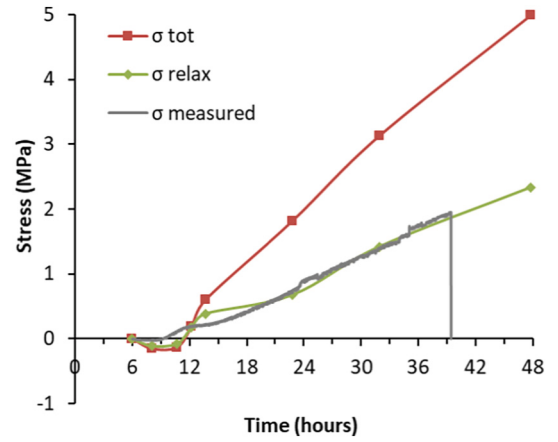
Fig. 15. Simulated stress of restrained AASC under semi-adiabatic condition. \sigma_{measured} is the measured stress as shown in Fig. 10.
