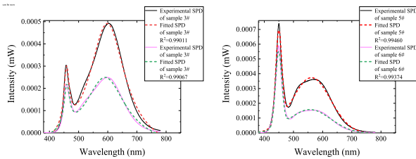
FIGURE 11. The experiment and fitted SPD of mid-power 3000K and 6000K white LEDs.
