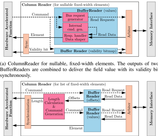
(b) List of fixed-width elements (non-nullable). Two BufferReaders are combined, where the offsets BufferReader provides a command for the values BufferReader. A list length stream and list element stream is provided to the computational kernel.
