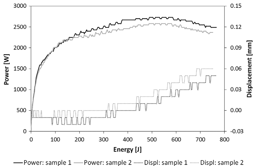
Figure 8 Representative power and displacement curves for two samples welded with 0.08 mm-thick EDs (1000 N welding force, 86.2 \mu\text{m} vibration amplitude, displacement-controlled welding). A positive displacement value corresponds to downward movement of the sonotrode
