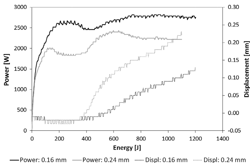
Figure 7 Representative power and displacement curves for 0.24 and 0.16 mm-thick EDs (1000 N welding force, 86.2 \mu m vibration amplitude, displacement-controlled welding). A positive displacement value corresponds to downward movement of the sonotrode
