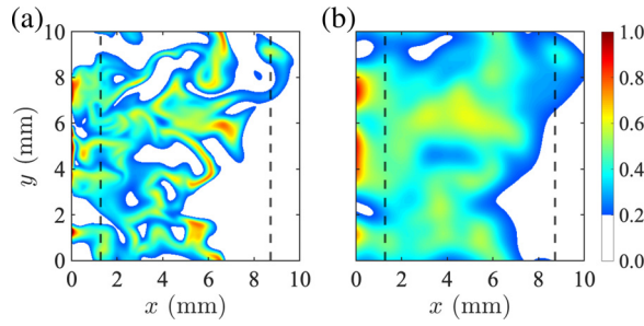
Fig. 1. Instantaneous (a) fully resolved reaction rate and (b) filtered reaction rate ( \Delta = \delta_{th,nom} ) of the case B1 in the mid-xy plane, normalized by using the maximum value. Dashed black lines denotes the sampling domain to avoid the open boundary effect on the filtering.
