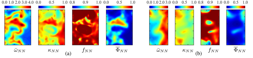
Fig. 8. Typical variations of \bar{\omega}_{NN} , \bar{\kappa}_{NN} , \bar{f}_{NN} and \bar{\Phi}_{NN} for B1 (a; \Delta/\delta_{th,nom} = 1.0 ) and BZ1 (b; \Delta/\delta_{th,nom} = 0.75 ).
