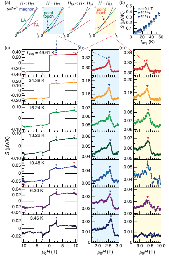
FIG. 3. (a) Magnon, TA-phonon, and LA-phonon dispersion relations for YIG when H < H_{TA} , H = H_{TA} , H_{TA} < H < H_{LA} , and H = H_{LA} . (b) T_{\text{avg}} dependence of the normalized SSE voltage S at \mu_0 H = 0.1 T, \mu_0 H_{TA} , and \mu_0 H_{LA} . (c) S(H) of the Pt/YIG/GGG sample for various values of T_{\text{avg}} in the range of |\mu_0 H| < 10.5 T. (d), (e) A blowup of S(H) around (d) H_{TA} and (e) H_{LA} .
