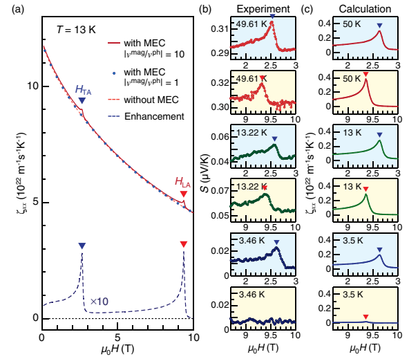
FIG. 4. (a) Calculated SSC \zeta_{xx} at T = 13 \text{ K} as a function of H , with (red solid curve and blue circles) and without (red dashed curve) magnetoelastic coupling (MEC). The red solid curve and the blue circles are computed for ratios of the scattering potentials of |v^{\text{mag}}/v^{\text{ph}}| = 10 and |v^{\text{mag}}/v^{\text{ph}}| = 1 , respectively. The blue dashed curve is a blowup of the difference between the red solid and dashed curves. (b) Experimental S and (c) theoretical \zeta_{xx} after subtraction of the zero MEC results.
