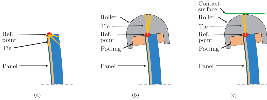
Fig. 4. Comparison of the three approximations of the roller boundary conditions: (a) method 1, panel only; (b) method 2, roller; (c) method 3, roller with contact.
