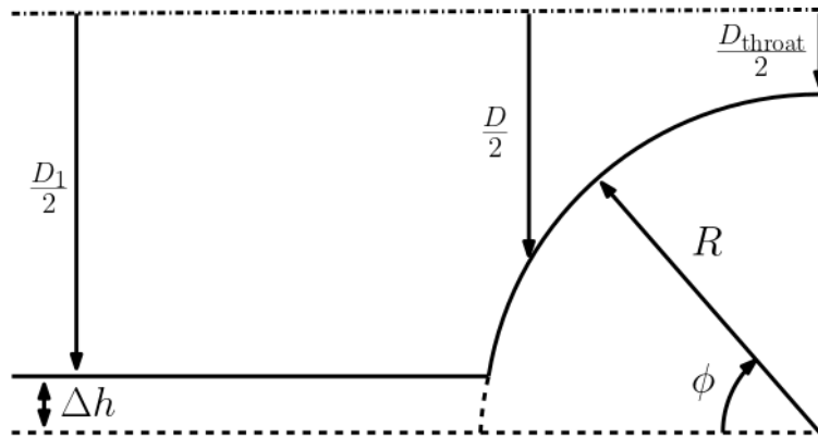
Fig. 10 Definition of square equivalent channel quantities. Where the dashed dotted line is a symmetry line.
