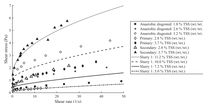
Fig. 19. Comparing rheograms of slurry 1 with primary and secondary sludge from (Markis et al., 2014) and anaerobic digested sludge from (Baudet et al., 2011).
