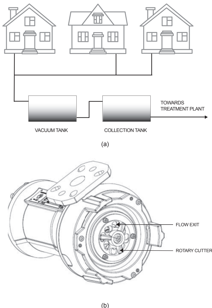
Fig. 2. a) Schematic drawing of a vacuum collection station. b) Cutter pump (submersible disintegrator pump manufactured by Landustrie).
