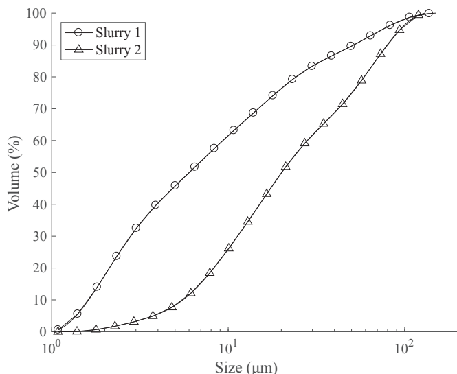
Fig. 3. Cumulative particle size distribution of slurry 1 and slurry 2.
