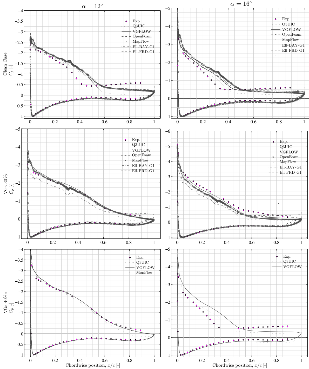
Figure 8: Pressure distributions for the NTUA T18 airfoil; C_p(x) for ( Left column ) \alpha = 12^\circ and ( right column ) \alpha = 16^\circ . Rows represent the Clean Case, VGs at 30%c and 40%c respectively. (Note different graph scale).
