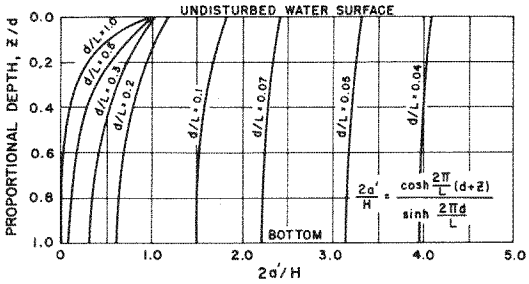
b. Horizontal amplitude of oscillation for proportional depth related to fraction of wave height.
