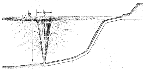
IDEALIZED SEWAGE FIELD DISCHARGE FROM VERTICAL OUTLET
