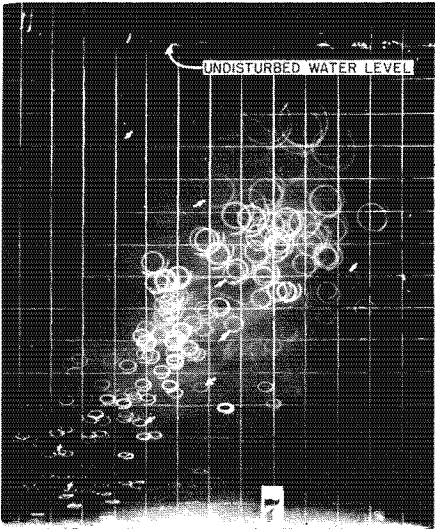
Fig. 6. Photograph of water particle orbits for a wave with the following dimensions. d = 2.50 feet, H = 0.339 feet, L = 6.42 feet, T = 1.12 seconds and d/L_0 = 0.39
