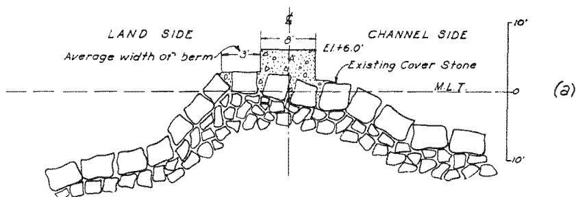
Section At Station 40+25 North Jetty - Showing Concrete Cap
