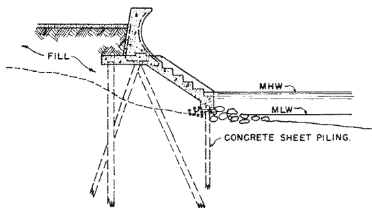
Fig. 5 Seawall -- combination.
