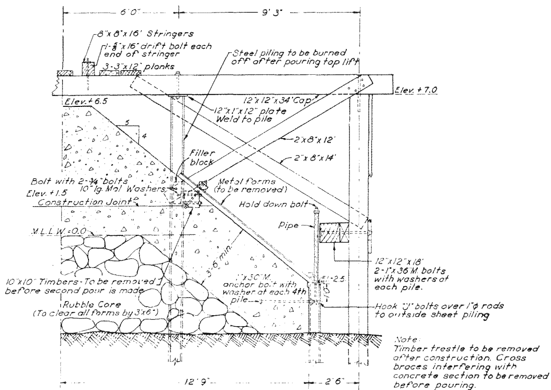
Fig. 3. Typical Section, Nome Harbor, Alaska -- West Jetty
