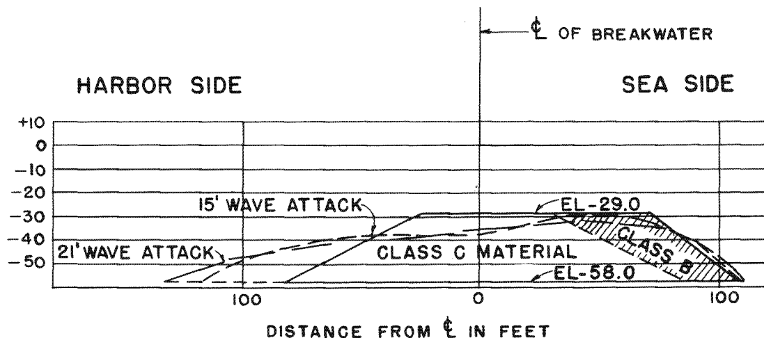
Fig. 15. Displacement of breakwater material by wave action.
