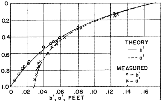
b. Comparison of measured orbit semi-major and semi-minor axes with theory: d/L_0 = 0.39
