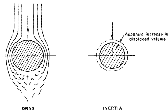
Fig. 2 Force components
