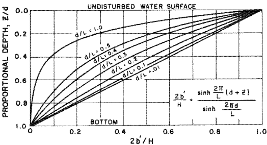
a. Vertical amplitude of oscillation for proportional depth related to fraction of wave height.
