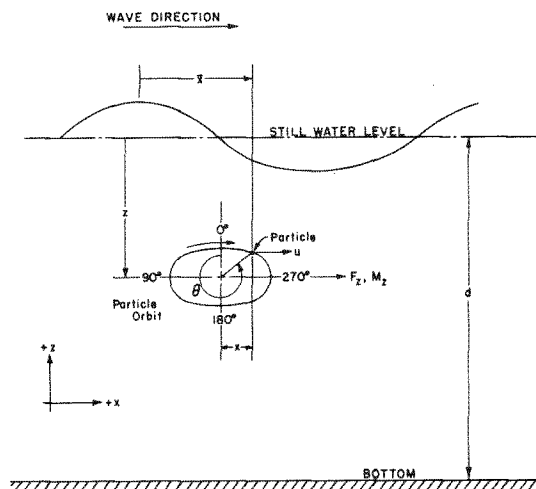
Fig. 1 Schematic diagram of particle motion
