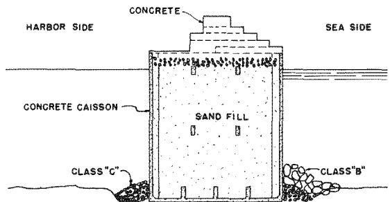
Fig. 9 Breakwater -- full caisson (modified vertical face).
