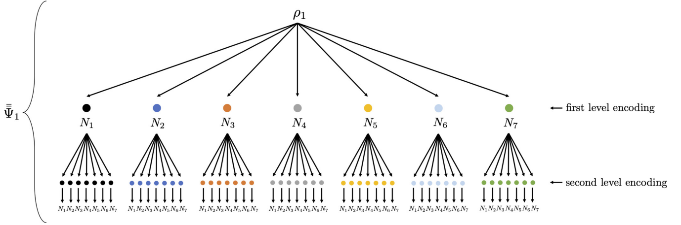
FIG. 2. Two-level encoding of the input qubit state \rho_1 of node 1. The double-encoded distributed state is denoted \bar{\Psi}_1 . Each circle represents a single-qubit share.
