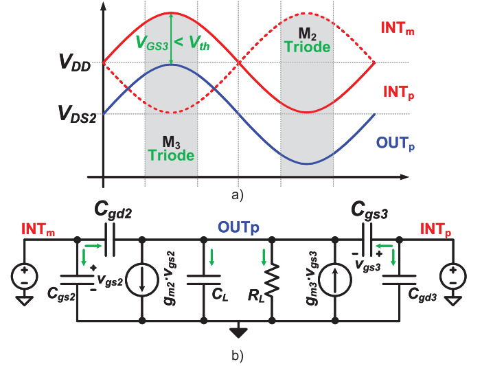
Fig. 5. DC-coupled low-voltage DCO output buffer. (a) Half-circuit large-signal excursions. (b) Half-circuit small-signal simplified model.
