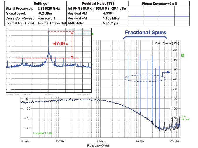
Fig. 17. Phase noise and spectrum closed-loop of RO-based ADPLL.
