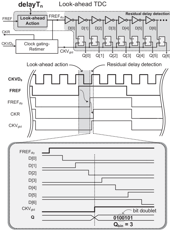
Fig. 7. Look-ahead TDC block diagram with interconnection to clock-gating and retiming circuitry along with all the signal waveforms.
