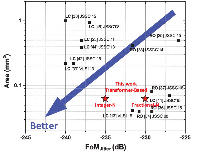
Fig. 20. FoM jitter over area for recent state-of-the-art fractional-N PLL.
