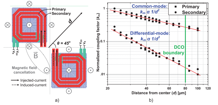
Fig. 1. Magnetic field cancellation. (a) Magnetic field directions. (b) Simulation of coupling factor ( k_m ) for common-mode and differential mode excitations.
