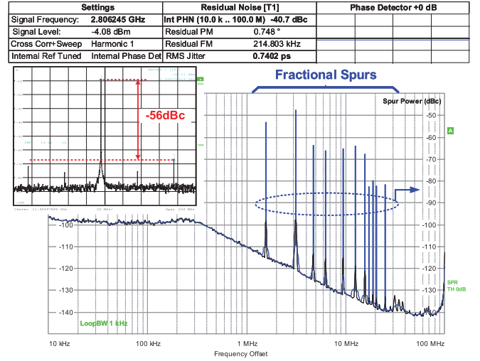
Fig. 16. Phase noise and spectrum closed-loop of transformer-based ADPLL.
