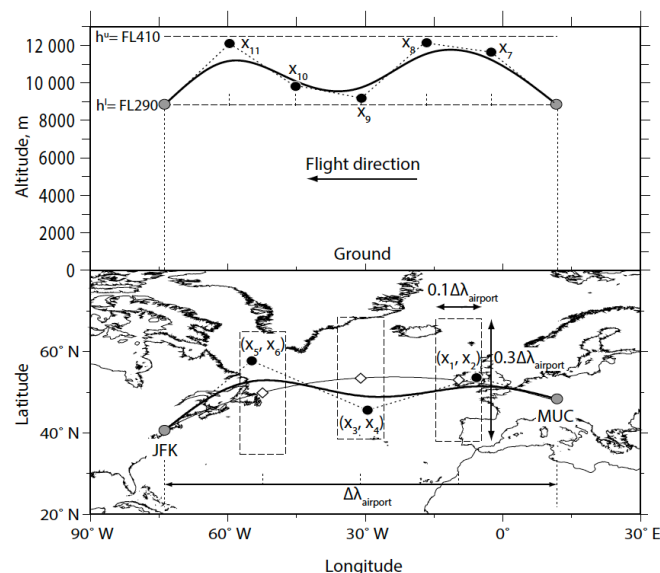
Figure 4. The geometry definition of a flight trajectory with the vertical cross section ( top ) and horizontal cross section ( bottom ) reprinted from [44]. The bold solid line indicates the real trajectory from MUC to JFK. The black dots are control points determined by design variables x_i . The cruise flight altitude is allowed to vary from 29,000 feet (FL290) to 41,000 feet (FL410). Bottom: the dashed boxes show rectangular domains of three control points. The diamonds along the great circle are centre points of the boxes. \Delta\lambda_{\text{airport}} is the longitudinal distance between two cities.
