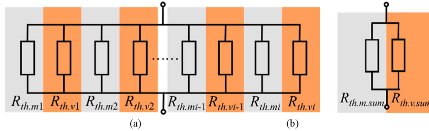
Fig. 5. (a) Thermal resistance network of nonhomogeneity layers; (b) Schematic of the thermal resistance of the same material after merging and combining.
