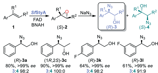
Fig. 5 One-pot chemo-enzymatic cascade from styrenes to chiral \alpha -azido alcohols, 15 mg scale, % isolated yield of product. Reaction conditions: [BNAH] = 30 mM, buffer (50 mM tris-SO 4 , pH 7.0), catalase (650 U mL -1 ), [FAD] = 50 \mu M, [ S /StyA] = 3 \mu M, [alkene] = 10 mM, [NaN 3 ] = 35 mM, final volume 10 mL, shaken in Erlenmeyer flasks on an incubator shaker at 180 rpm and 30 °C for 22 h.
