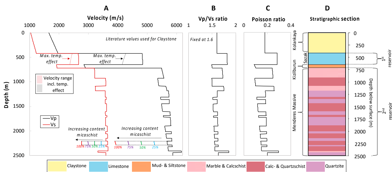
Figure 16. Seismic velocity profiles (A), P-wave/S-wave velocity ratio, i.e., V_p/V_s (B), Poisson ratio (C), and the stratigraphic section of interest (D). The stratigraphic section represents the planned CO 2 injection site at the Kızıldere geothermal reservoir. For the intervals that contain multiple rock types (mud- and siltstone, marble and calcschist, and calc- and quartzschist), a 50/50 distribution was assumed. Velocity–depth relationships, i.e., linear regressions, from Figure 8 (P-wave) and Figure S6 (S-wave) were used to construct the profile shown in (A). Since the claystone could not be assessed in this study, a literature value for its P-wave velocity, and for its V_p/V_s ratio, was assumed [67]. In one calc- and quartzschist layer, micaschists were added in varying degrees (25, 50, 75, and 100%) to show its effect on the resulting velocities. Note that the velocity profiles presented (black and red profiles in (A)) reflect only the stress-dependency of the seismic velocities for dry conditions. In order to give an impression of the effect of temperature, on related velocities, the maximum temperature effect (dashed red and black profiles in (A)) was added for the limestone interval. This represents the reduction in velocity with increasing temperature at atmospheric pressure (as presented in Figure 12 and Figure S8). It is expected that the real dry velocity of the limestone interval in (A) lies somewhere in between the dashed and continuous lines, as it is assumed that the temperature-dependency is highest at atmospheric conditions, hence the ‘maximum temperature effect’.
