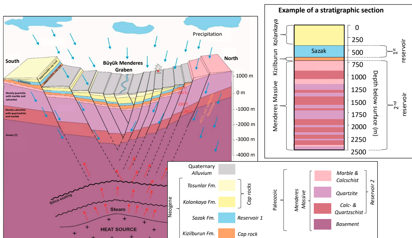
Figure 1. Left: Kızıldere geothermal field conceptual model using the most recent reservoir classification (revised after [33]). Right: Example of a stratigraphic section, revealing the actual formation sequence represented by the three different lithologies that make up the second reservoir.
