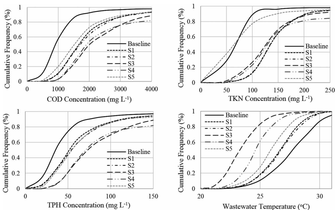
Figure 4 | Variation in wastewater quality parameters (COD, TKN, TPH concentration and wastewater temperature) obtained with the stochastic water quality model at the catchment outfall.
