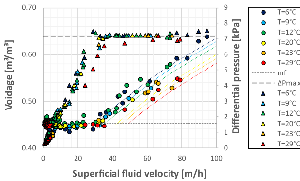
Fig. 6. Up-flow filtration and expansion curve for rapid filter sand granules 0.8 < d_p < 1.25 mm. Experimental voidage (circles), Carman-Kozeny predicted voidage (●●●) and differential pressure (triangles) against superficial fluid velocity, (---) maximum pressure drop, (—) voidage at minimum fluidisation.
