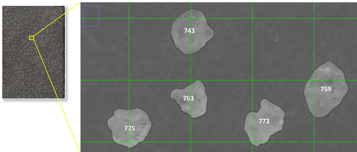
Fig. 3. Scanned sample with particle analysis with ImageJ, with particle outlines and particle numbers, with 2 \times 2 mm gridlines.
