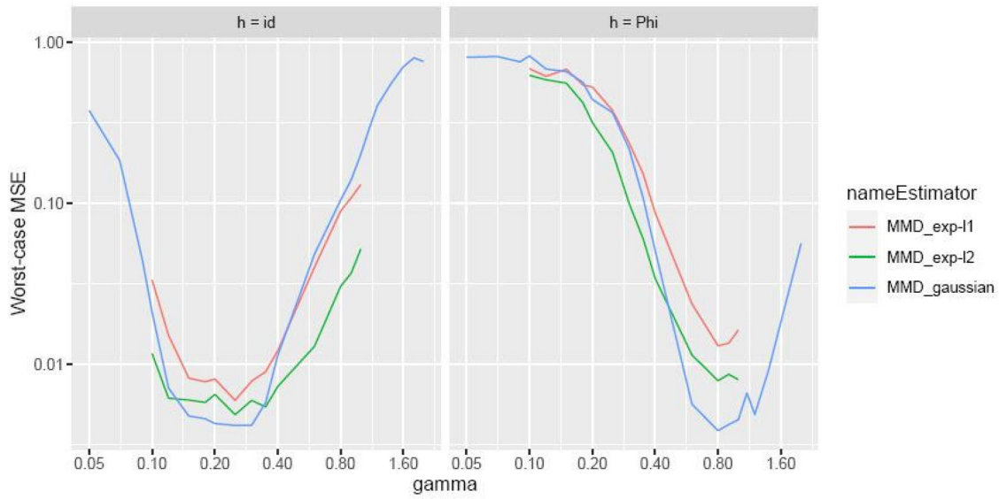
Figure 1. MSE of \hat{\theta}_h based on the Gaussian kernel k_U(U, V) = \exp(-\|h(U) - h(V)\|_2^2/\gamma^2) , the exp-L 2 kernel k_U(U, V) = \exp(-\|h(U) - h(V)\|_2/\gamma) and the exp-L 1 kernel k_U(U, V) = \exp(-\|h(U) - h(V)\|_1/\gamma) , as functions of \gamma .
