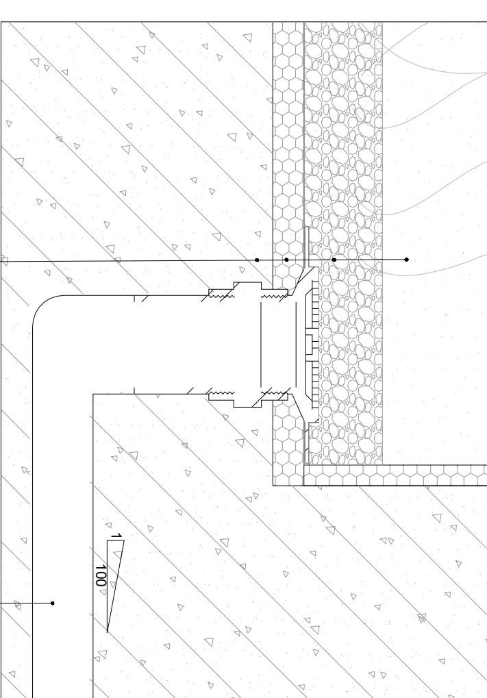
Detail 04/ 1:5
