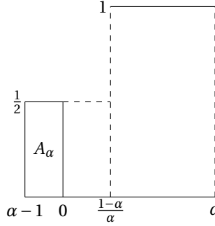
Figure 3.2: \Omega_\alpha, \alpha = 0.8
