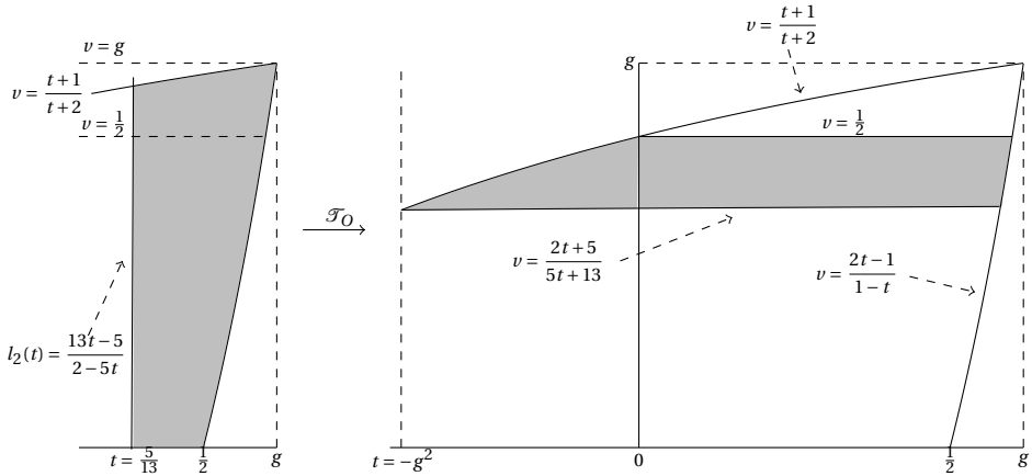
Figure 2.6: The map of the rightmost strip applying \mathcal{T}_O
