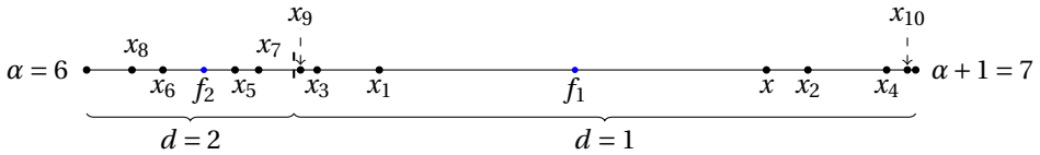
Figure 4.3: N = 50, \alpha = 6, x = 6.8
