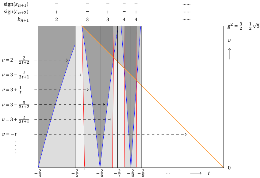
Figure 2.13: The patterns \mathcal{A} through \mathcal{F} for \epsilon_{n+1} < 0
