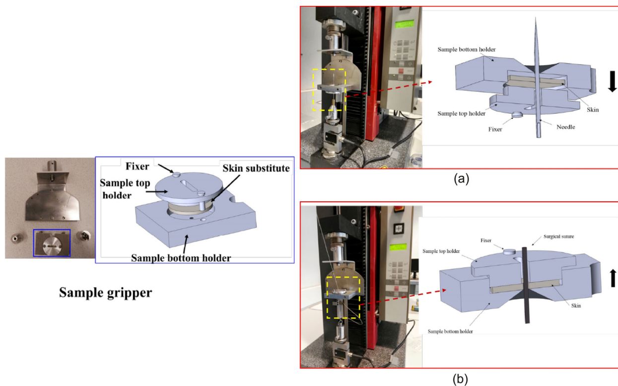
Fig. 3 Penetration friction apparatus (PFA). (a) punch process; (b) penetration process.
