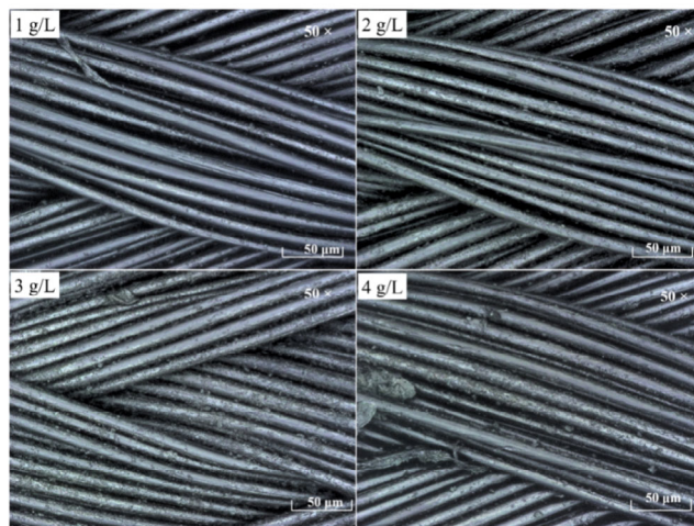
Fig. 9 Morphologies of the surfaces of the PGA multifilament surgical sutures for different DA concentrations ranging from 1 g/L to 4 g/L at a pH of 8.5 (magnification 50×; one pixel represents 0.135 mm × 0.135 mm).
