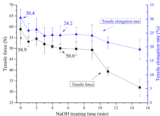
Fig. 6 Tensile force and elongation rate of the PGA surgical sutures after NaOH treatment.
