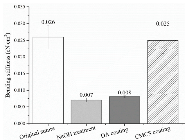
Fig. 14 Bending stiffness of PGA multifilament surgical suture with different treatments.
