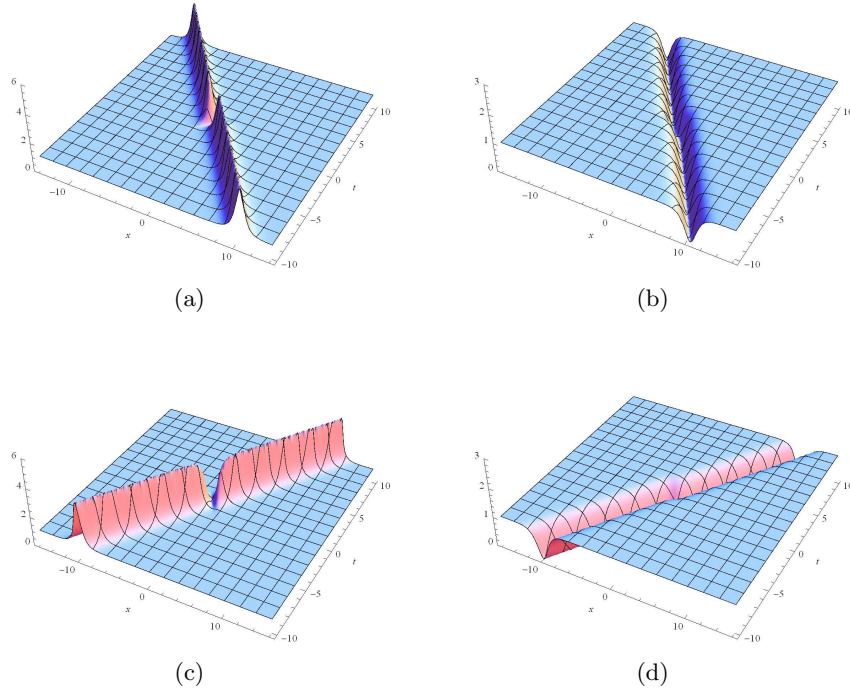
Fig. 7. Interactions of X_1 - X_2 solitons with degeneration: shape and motion of the envelope |q|^2 resulting from (102). (a) 3D plot for b = 0.5, \beta = 0.5 - \frac{\sqrt{3}}{2}i . (b) 3D plot for b = 0.5, \beta = -0.5 + \frac{\sqrt{3}}{2}i . (c) 3D plot for b = 0.5, \beta = -0.5 . (d) 3D plot for b = 0.5, \beta = 0.5 . In (a) and (b), X_2 -soliton vanishes in the background |q|^2 = 1 . In (c) and (d), X_1 -soliton vanishes in the background |q|^2 = 1 .
