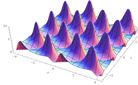
Fig. 8. Envelope of doubly periodic solution (103) for the defocusing reverse-space NLS equation (100), for b = -1.25, \beta = 1 .
