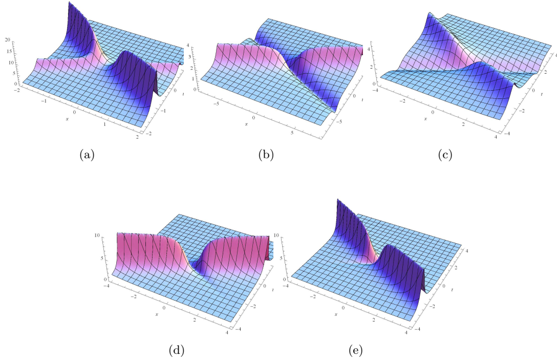
Fig. 9. Interactions of the X_1 - X_2 solitons for the defocusing reverse-space NLS equation (100): shape and motion of the envelope |q|^2 resulting from (110). (a) 3D plot for \hat{d} = 0.5 . (b) 3D plot for \hat{d} = -2i . (c) 3D plot for \hat{d} = 0.2 - 0.5i . (d) 3D plot for \hat{d} = 0.5 - i . (e) 3D plot for \hat{d} = 0.5 - 0.5i . In (a), (b) and (c), the branch in up-right direction stands for the X_2 -soliton, the other is for the X_1 -soliton. In (d), X_1 -soliton vanishes in the background |q|^2 = 1 . In (e), X_2 -soliton vanishes in the background |q|^2 = 1 .
