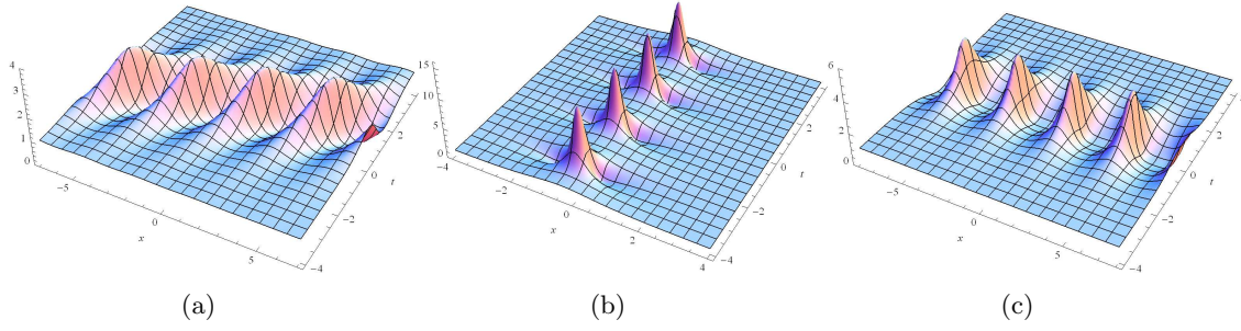
Fig. 1. Shape and motion of one breather solution of the focusing NLS equation (1) with a background solution q_0 = e^{-2it} . The envelope is given by (73) where f is (77). (a) 3D-plot for a moving breather associated with (80) for a_1 = 0.3, b_1 = -0.3, \xi_{1R}^{(0)} = \xi_{1I}^{(0)} = 0 . (b) 3D-plot for the Kuznetsov-Ma breather associated with (82) for a_1 = 1.2, \xi_{1R}^{(0)} = \xi_{1I}^{(0)} = 0 . (c) 3D-plot for the Akhmediev breather associated with (83) for a_1 = 0.5, \xi_{1R}^{(0)} = \xi_{1I}^{(0)} = 0 .
