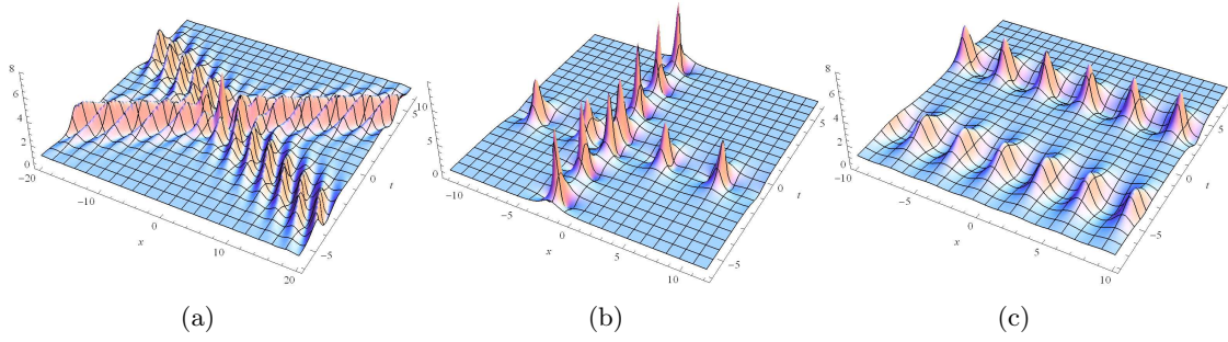
Fig. 2. Shape and motion of two-breather interactions of the focusing NLS equation (1) with a background solution q_0 = e^{-2it} . The envelope is given by (73) where f is (84). (a) 3D-plot for a_1 = 0.3, b_1 = 0.5, a_2 = 0.3, b_2 = -0.5, \xi_{1R}^{(0)} = \xi_{1I}^{(0)} = \xi_{2R}^{(0)} = \xi_{2I}^{(0)} = 0 . (b) 3D-plot for a_1 = 1.2, b_1 = 0, a_2 = 0.8, b_2 = 0, \xi_{1R}^{(0)} = 1, \xi_{1I}^{(0)} = 0, \xi_{2R}^{(0)} = 1, \xi_{2I}^{(0)} = 0 . (c) 3D-plot for a_1 = 0.3, b_1 = 0, a_2 = 0.5, b_2 = 0, \xi_{1R}^{(0)} = 2, \xi_{1I}^{(0)} = 0, \xi_{2R}^{(0)} = -2, \xi_{2I}^{(0)} = 0 .
