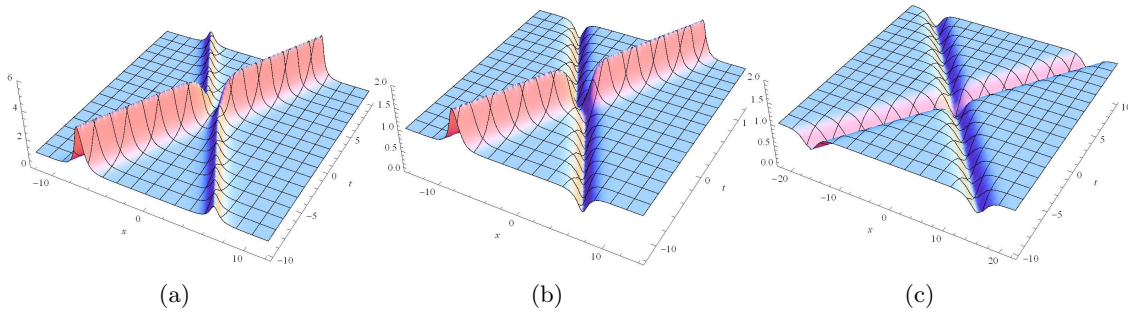
Fig. 6. Interactions of the X_1 - X_2 solitons for the defocusing reverse-space NLS equation (100): shape and motion of the envelope |q|^2 resulting from (102). (a) 3D plot for b = 0.3, \beta = -1.6 - 0.4i . (b) 3D plot for b = 0.3, \beta = -0.5 + 0.1i . (c) 3D plot for b = -0.8, \beta = 1.4 - i . In (a) and (b), X_2 -soliton is the branch in up-right direction, and the other is X_1 -soliton. In (c) X_1 -soliton is the branch in up-right direction, and the other is X_2 -soliton.
