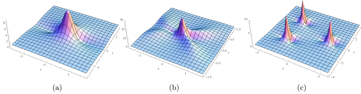
Fig. 4. Shape and motion of rational solutions of the focusing NLS equation (1). (a) Envelope of the first order rational solution given by (93) with s_0 = 1, s_1 = 0.5 . (b) Envelope of the second order rational solution given by (94) with s_0 = 2, s_1 = 0.5 . (c) Envelope of the second order rational solution given by (94) with s_0 = 1, s_1 = 0, s_2 = 10, s_3 = -20 .
