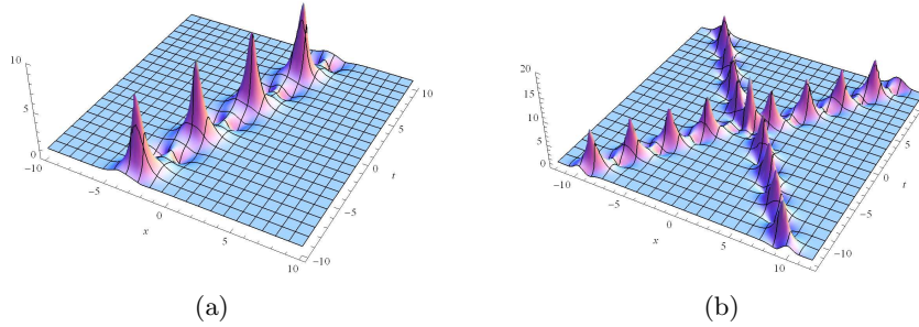
Fig. 11. Shape and motion of the envelope |q|^2 of the nonlocal defocusing reverse-space-time NLS equation (120). (a) 3D-plot for the one breather resulting (125) with k_1 = 0.3 - 0.15i . (b) 3D-plot for two breathers interaction resulting from (123) with k_1 = 0.5 + 0.3i, k_2 = 0.5 - 0.3i, \hat{c}_1^\pm = \hat{c}_2^\pm = 1 .
