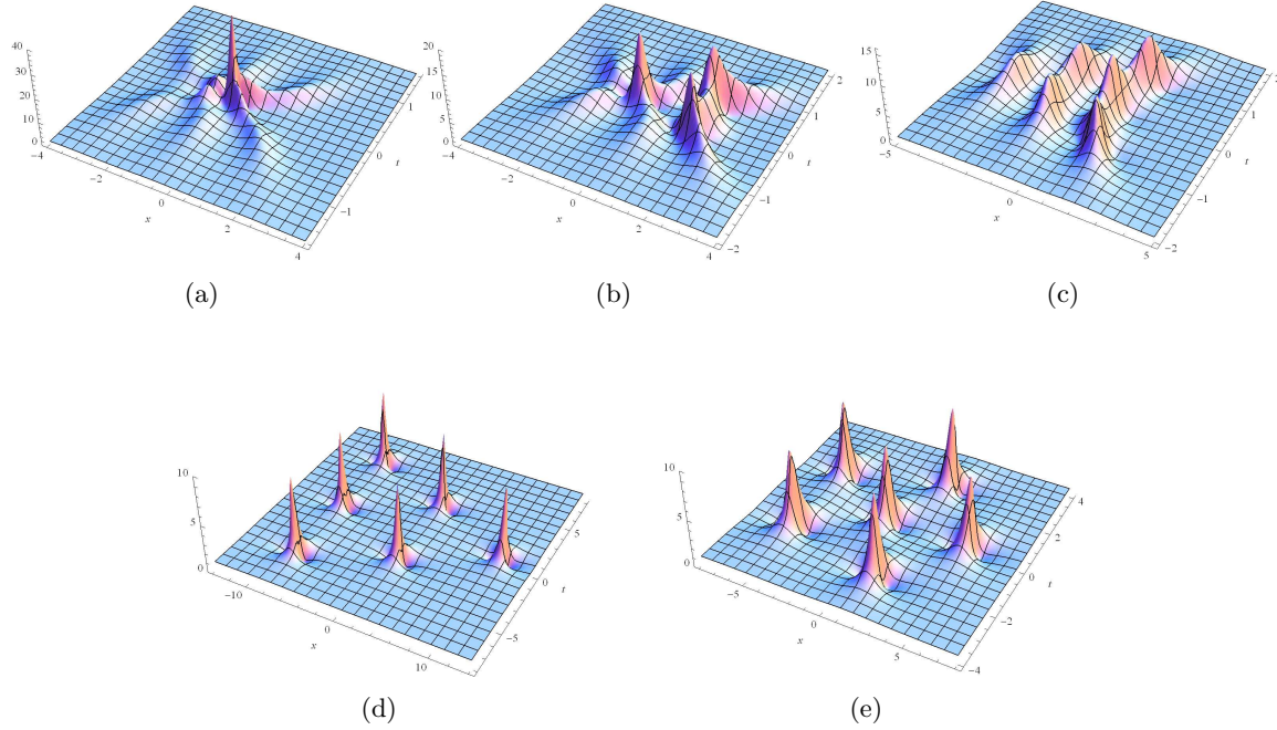
Fig. 5. Shape and motion of the envelope of the third order rational solution of the focusing NLS equation (1). (a) 3D plot for s_0 = 1, s_1 = 0, s_2 = 0, s_3 = 0, s_4 = 0, s_5 = 0 . (b) 3D plot for s_0 = 1, s_1 = 1, s_2 = 0, s_3 = 0, s_4 = 0, s_5 = 0 . (c) 3D plot for s_0 = 1, s_1 = 0, s_2 = 0, s_3 = 1, s_4 = 0, s_5 = 0 . (d) 3D plot for s_0 = -1, s_1 = 0, s_2 = 0, s_3 = 100, s_4 = -200, s_5 = 0 . (e) 3D plot for s_0 = 1, s_1 = 0, s_2 = 100, s_3 = 1, s_4 = 0, s_5 = 200 .
