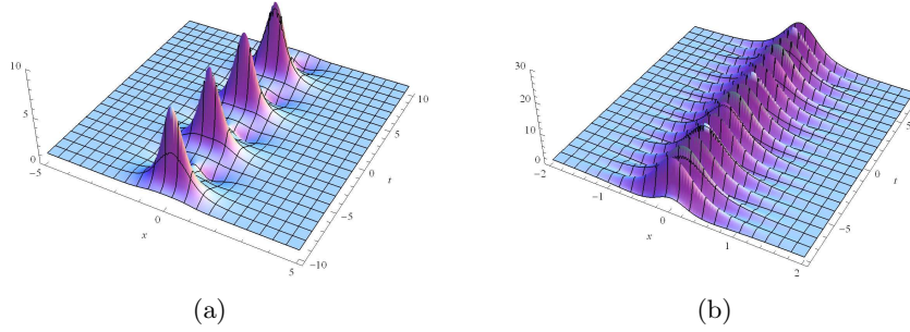
Fig. 10. Shape and motion of stationary breather of |q|^2 resulting from (124) for the nonlocal defocusing reverse-space-time NLS equation (120). (a) 3D-plot for k_1 = 0.3 . (b) 3D-plot for k_1 = 1 .
