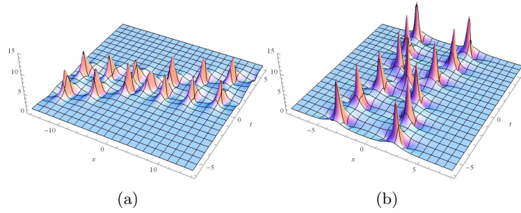
Fig. 3. Shape and motion of Jordan block solution of the focusing NLS equation (1) with a background solution q_0 = e^{-2it} . The envelope is given by (73) where f is composed by (85). (a) 3D-plot for a_1 = 0.8, b_1 = -0.15, \xi_{1R}^{(0)} = \xi_{1I}^{(0)} = 0 . (b) 3D-plot for a_1 = 1.2, b_1 = 0, \xi_{1R}^{(0)} = \xi_{1I}^{(0)} = 0 .
