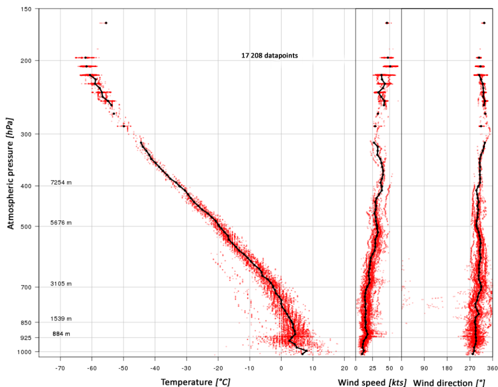
Figure 13. Temperature and wind profile on 21 April 2016 at 09:00 UTC, based on Mode S transponder data derived with an ADS-B receiver of ascending and descending aircraft in the vicinity of the two Berlin airports (Bütow, 2016).
