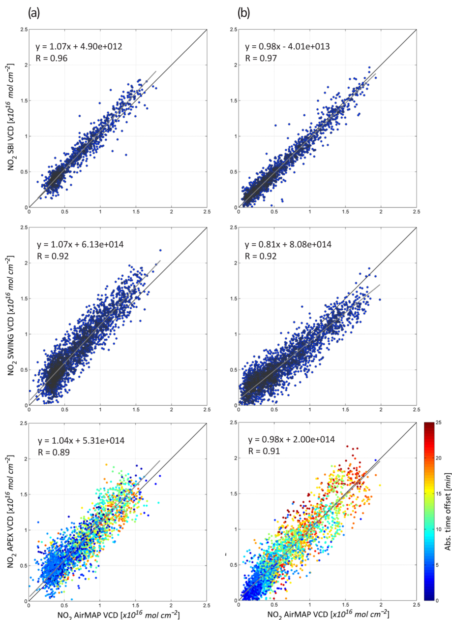
Figure 19. Scatter plots and orthogonal linear regression analyses of the co-located \text{NO}_2 VCDs, retrieved from the harmonised maps for respectively (a) the morning and (b) afternoon flights on 21 April 2016. The AirMAP \text{NO}_2 VCDs are plotted on the x axis. The black solid line and grey line represent the 1 : 1 ratio and the linear regression, respectively. The colour-coding in the lower plots indicates the absolute time offset between the observations from the two aircraft. Note that the same data points are plotted as in the time series plots of Fig. 18.
