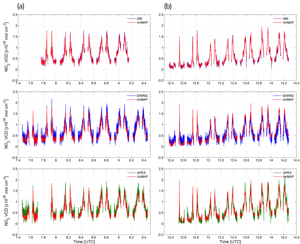
Figure 18. Co-located \text{NO}_2 VCDs retrieved from the harmonised maps for respectively (a) the morning and (b) afternoon flights on 21 April 2016. APEX VCDs are provided in green, AirMAP in red, SWING in blue, and SBI in purple. The x axis corresponds to the acquisition time, recorded by the Cessna 207T D-EAFU.
