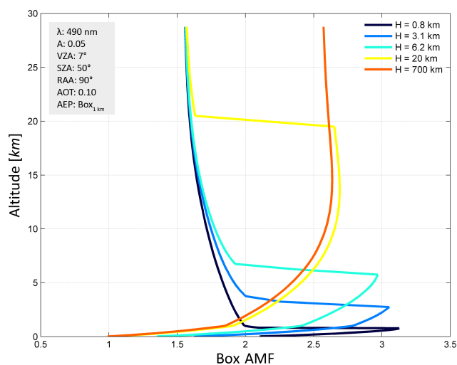
Figure 8. Height-dependent box AMFs assessing the vertical sensitivity to NO 2 , illustrated for five different scenarios for the sensor altitude H , in kilometres above ground level.
