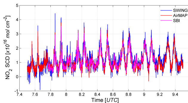
Figure 3. Time series of averaged NO 2 near-nadir SCDs (> −4 and < 4° VZA), retrieved from AirMAP, SWING, and SBI observations, during the morning flight over Berlin on 21 April 2016.
