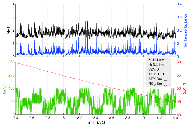
Figure 6. Time series of \text{NO}_2 AMFs for the morning flight on 21 April 2016, computed with DISORT based on the RTM parameters from the AirMAP instrument. The data are plotted for only the nadir observations in each across-track scan line.
