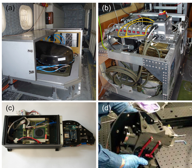
Figure 2. Overview of the four DOAS imaging instruments: APEX (a), AirMAP (b), SWING (c), and SBI (d).
