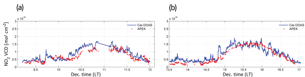
Figure 14. APEX and car DOAS \text{NO}_2 VCD time series for (a) the morning and (b) afternoon flights on 21 April 2016, respectively.
