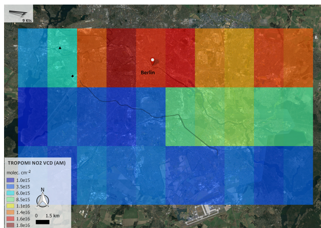
Figure 20. Tropospheric NO 2 VCDs retrieved from AirMAP for the morning flight over Berlin on 21 April 2016 (Google, TerraMetrics) and gridded at the spatial resolution of the TROPOMI spaceborne instrument (3.5 by 7 km 2 ). The key contributing NO 2 emission sources are indicated by a black triangle (power plant Reuter West) and black diamond (Messe Berlin). The highways A100 and A113, running south of the city, are marked by the grey line. Hourly averaged wind vectors indicate the surface wind at 08:00 (light grey, 3.3 m s -1 ), 09:00 (grey, 4.9 m s -1 ), and 10:00 (black, 5.1 m s -1 ) UTC. The average surface wind speed is indicated on the maps. A pattern of enhanced NO 2 with clear gradients can be observed, originating from the Berlin city region. However, the two main west-east-oriented plumes cannot be spatially resolved anymore at the spatial resolution of TROPOMI. Note as well that only a slight NO 2 enhancement is observed for the pixel containing the main sources, i.e. the power plant Reuter West and Messe Berlin. The plumes are narrow and confined close to the source and the particular pixel contains a considerable number of background values smoothing out the elevated levels of NO 2 .
