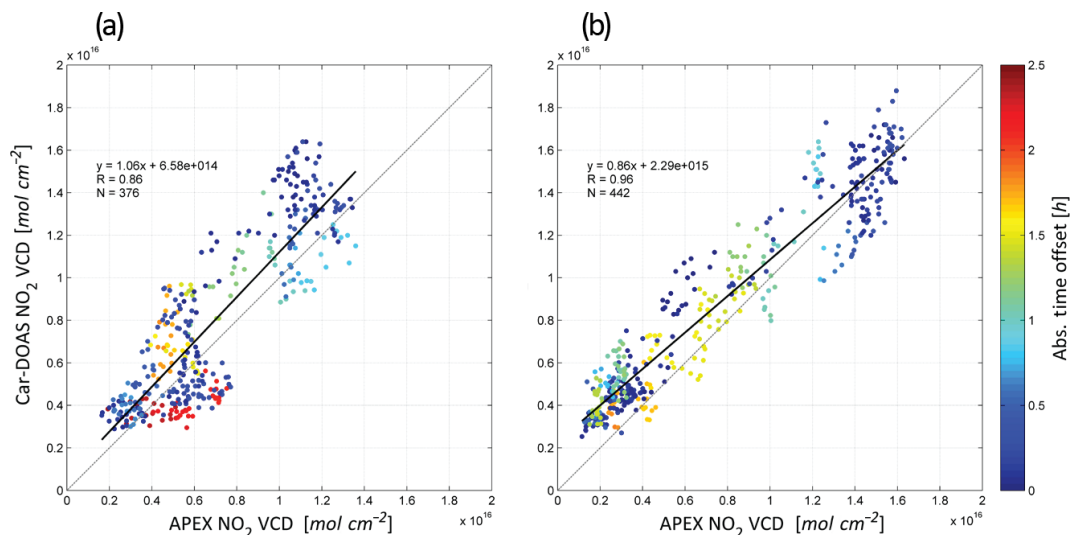
Figure 15. Scatter plots and linear regression analyses of the co-located \text{NO}_2 VCDs, retrieved from APEX and car DOAS for (a) the morning and (b) afternoon flights on 21 April 2016, respectively. Data points are colour-coded based on the absolute time offset between APEX and car DOAS observations.
