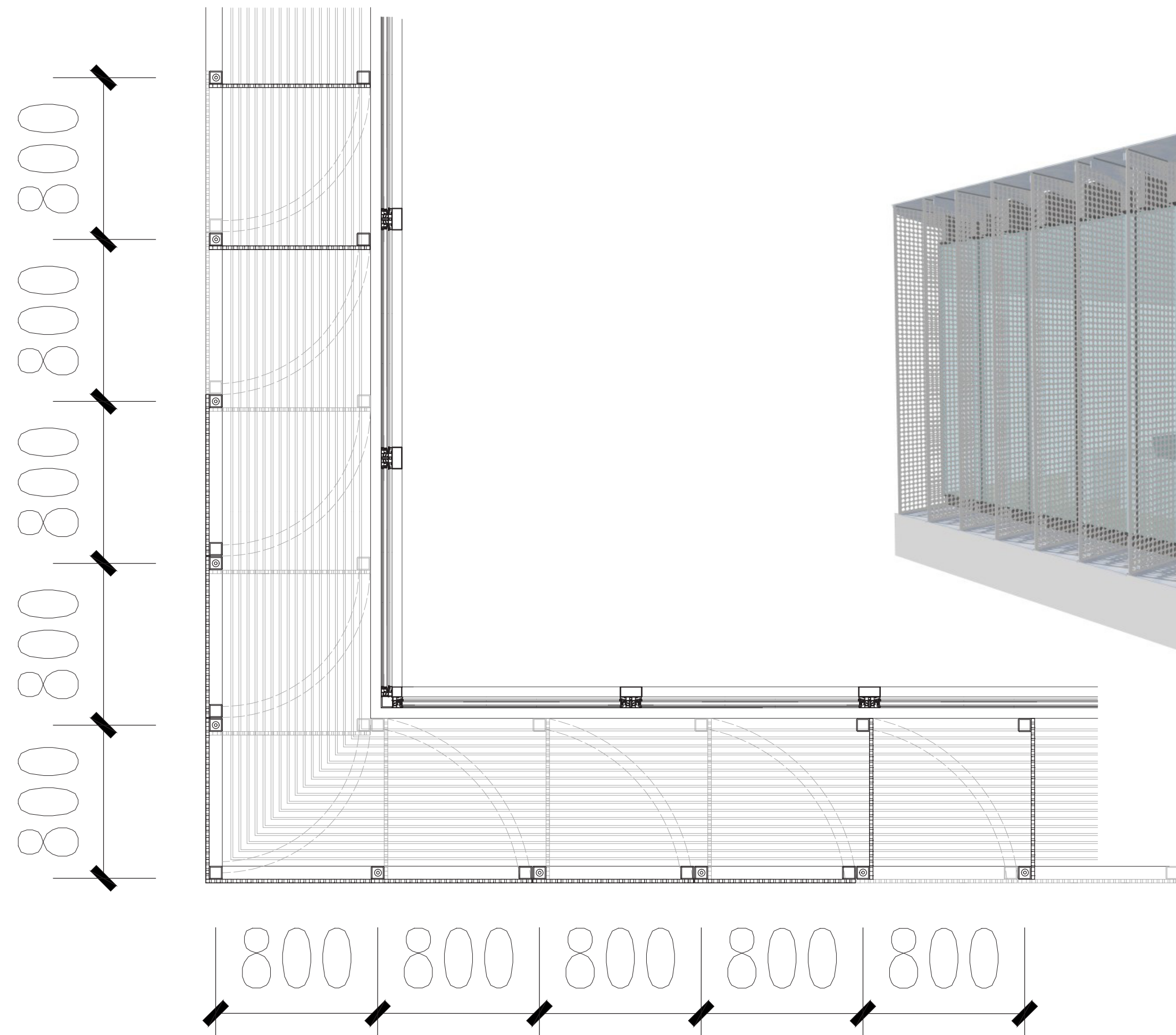
FACADE FRAGMENT VERT(UPPER PART) | SCALE 1:20
