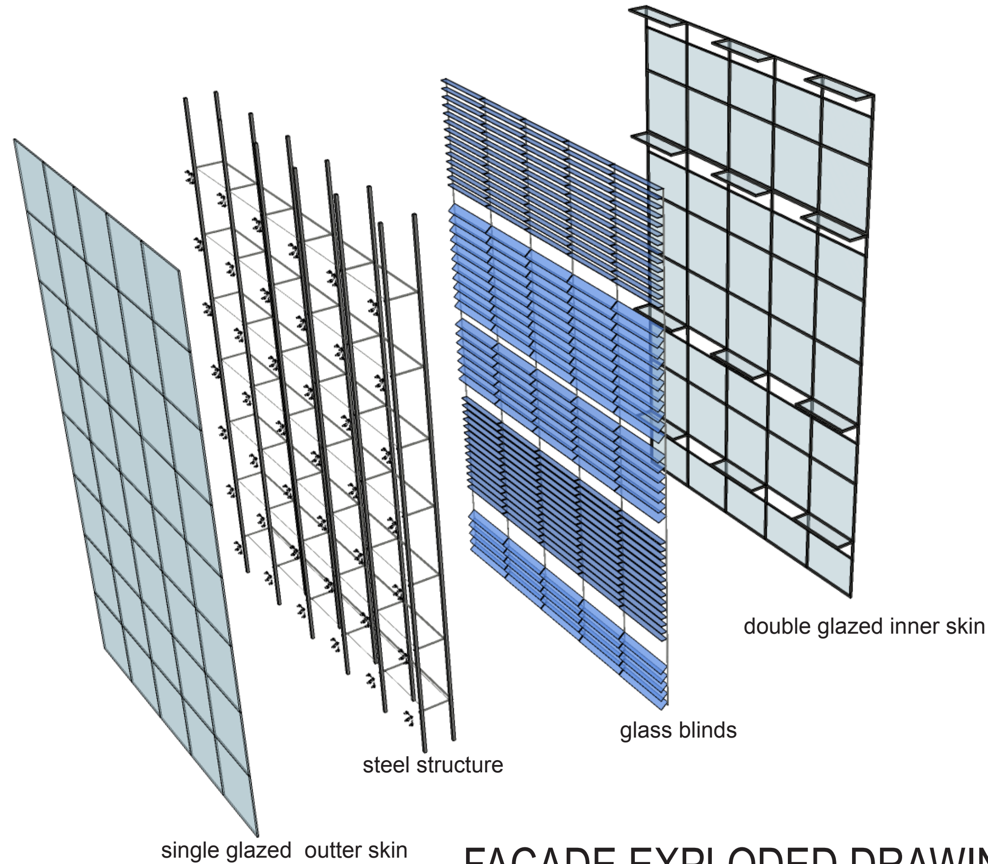
FACADE EXPLODED DRAWING
