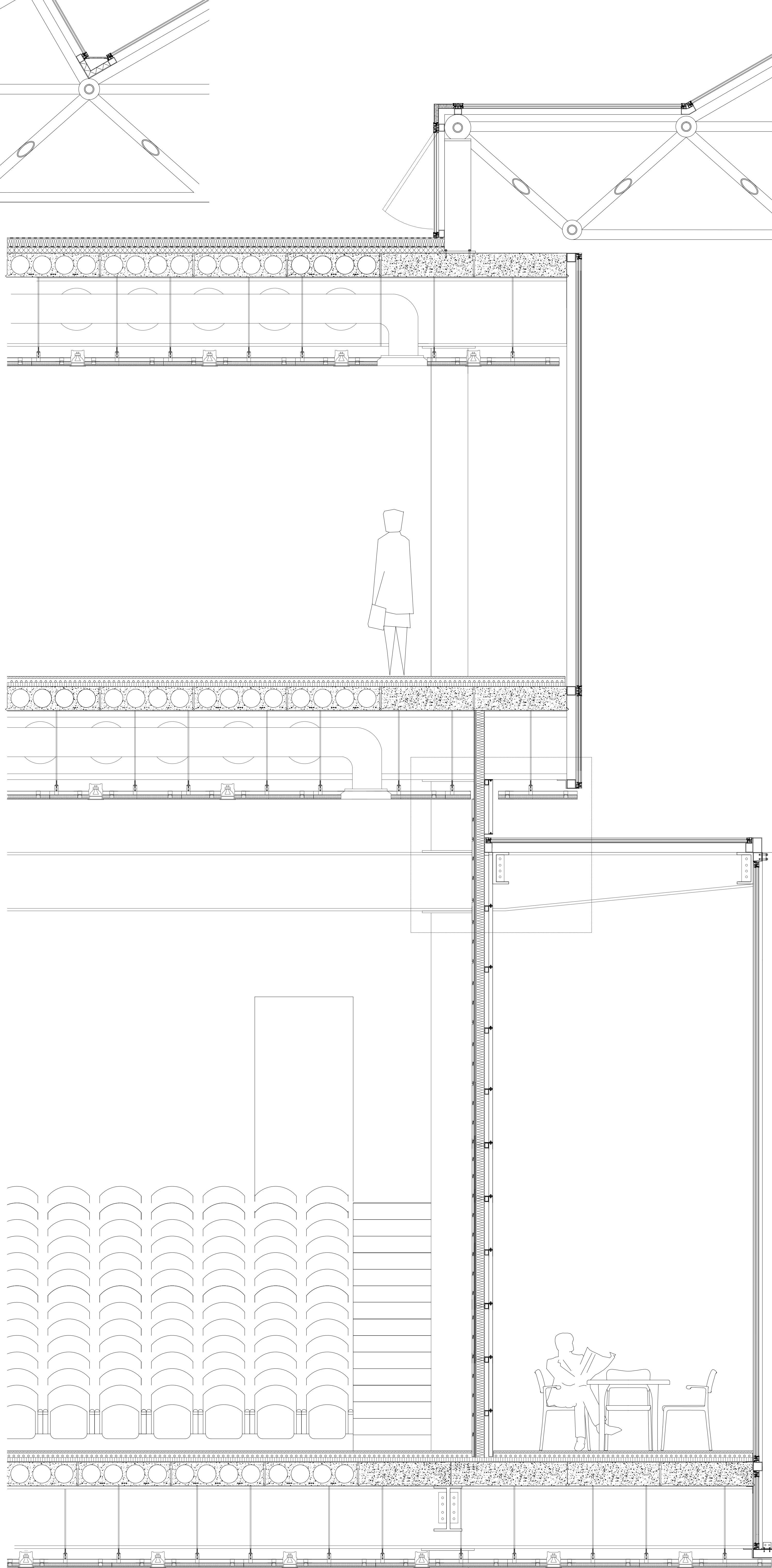
PARTS OF THE BUILDING | OFFICE AND AUDITORIUMS | SCALE 1:20
