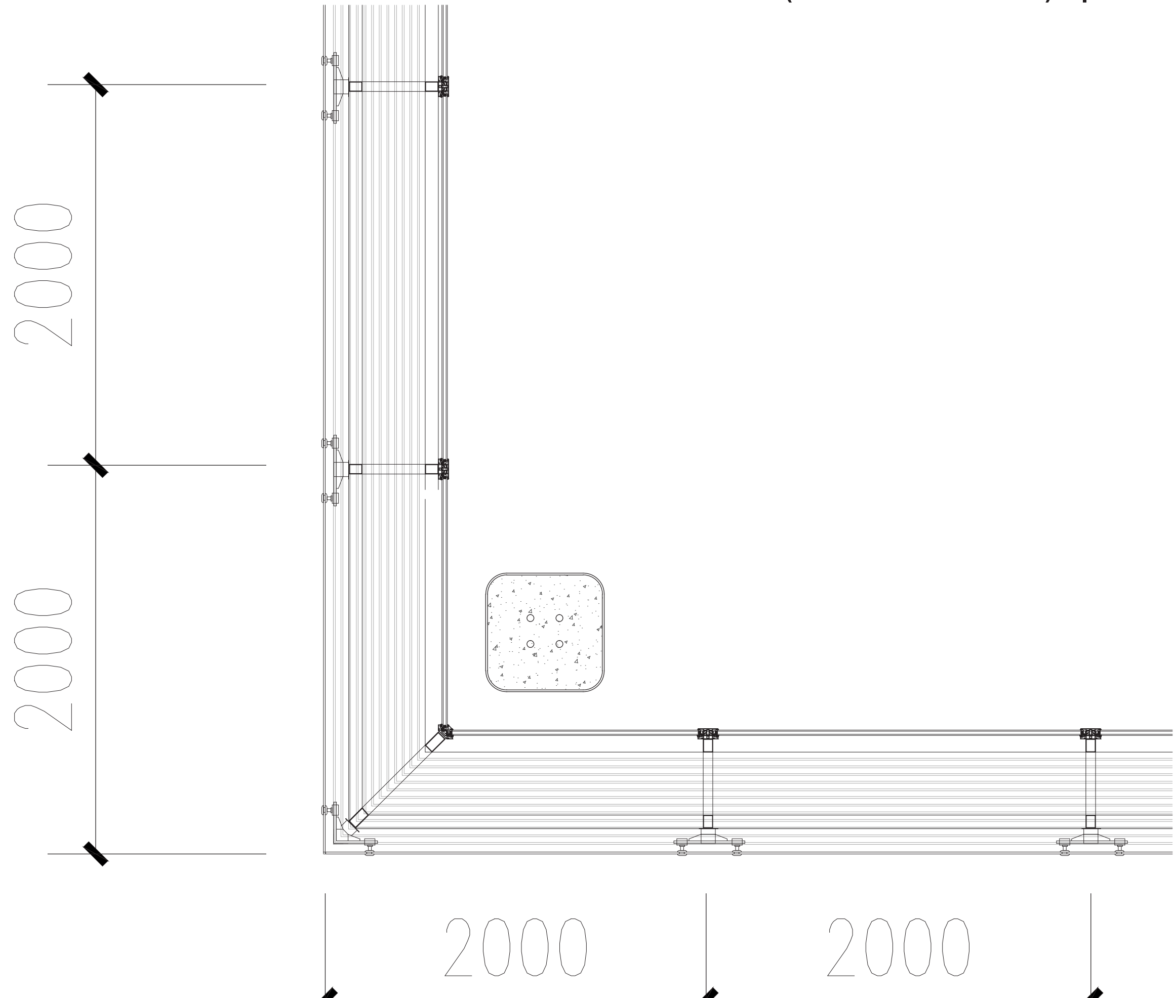
FACADE FRAGMENT VERT(LOWER PART) | SCALE 1:20
