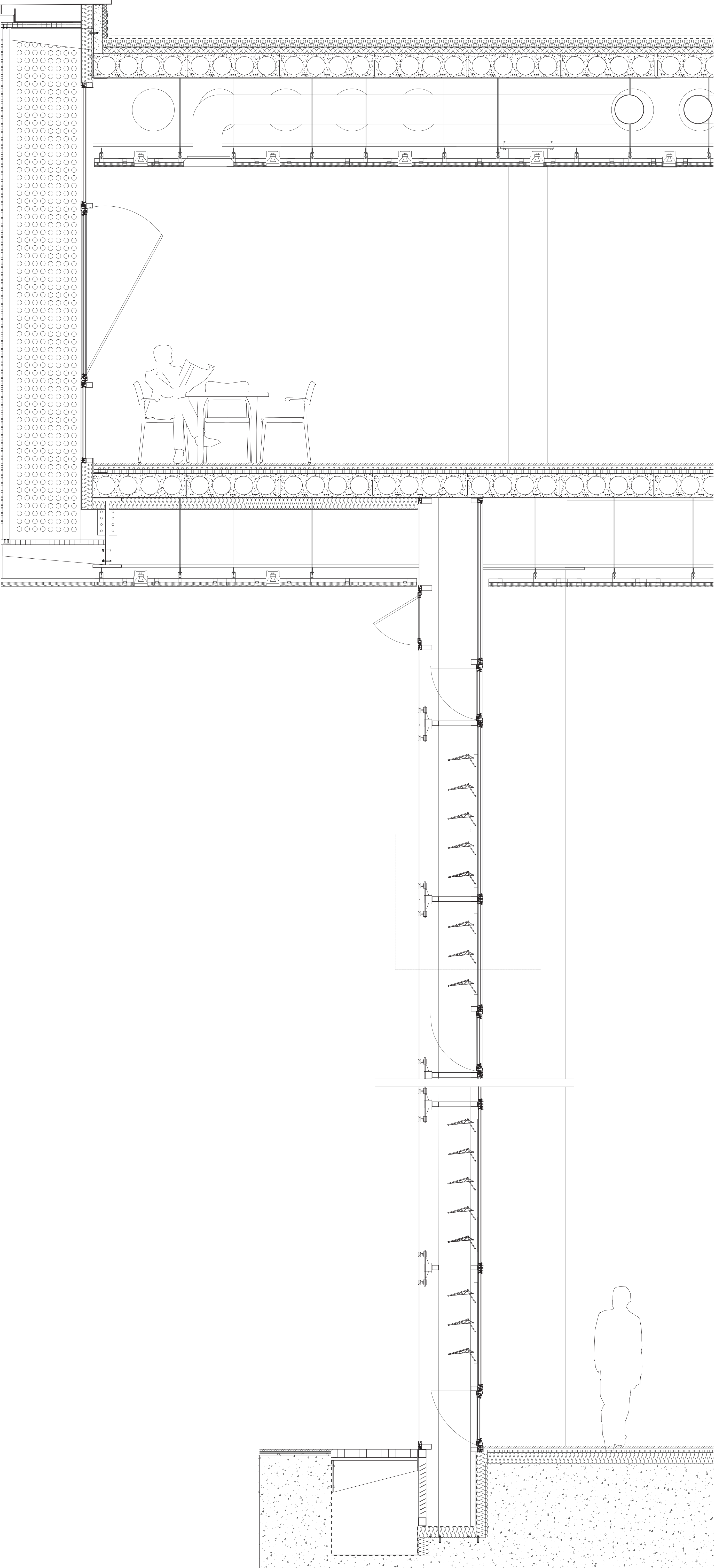
FACADE FRAGMENT HOR | SCALE 1:20
