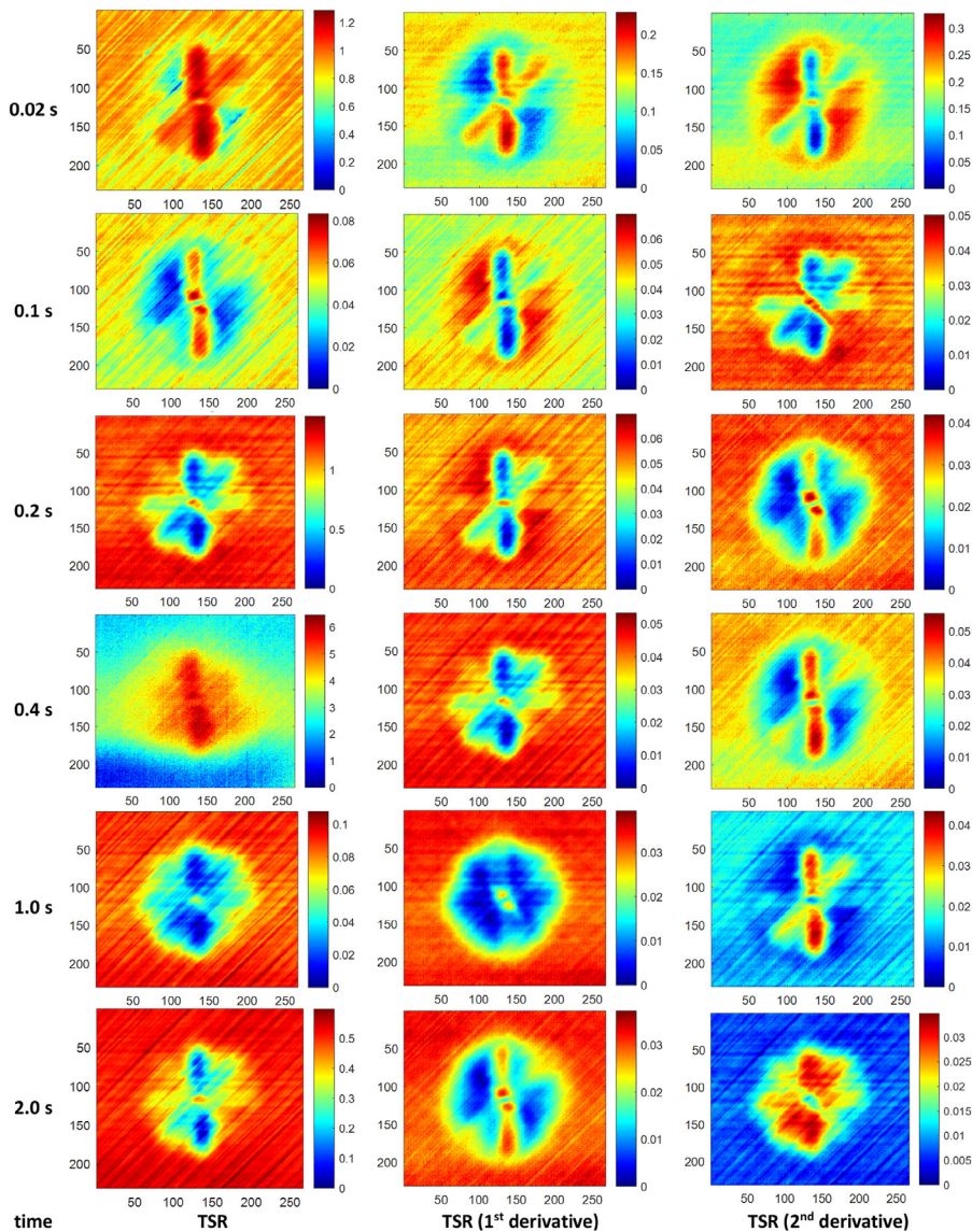
Figure 8.5 Results of TSR and its first and second derivatives for the first CFRP sample at various times.
