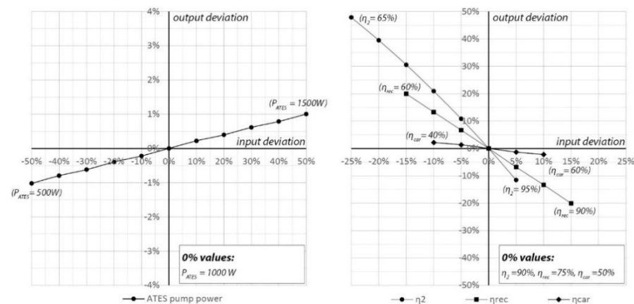
Figure 9. Sensitivity analysis of four parameters. Left: P_{ATES} . Right: \eta_2 , \eta_{rec} and \eta_{car} .
