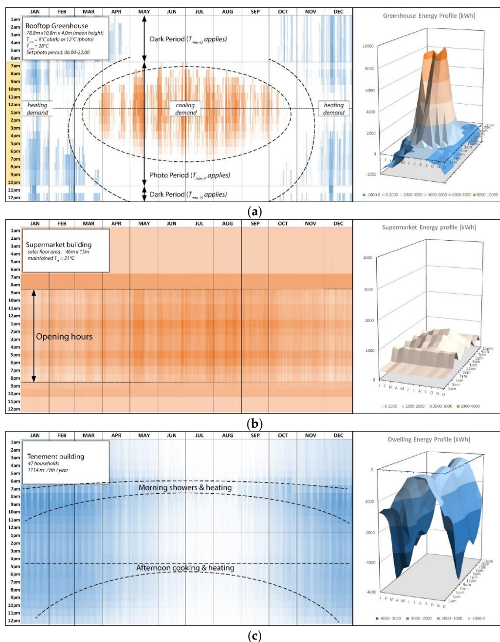
Figure 3. (a) Greenhouse: the energy profile of the greenhouse shows a white transition zone when the greenhouse indoor temperature is within the desired range. Temperature set points and photo-period used for the initial situation are mentioned in the figure. (b) Supermarket energy balance: The supermarket has a year-round cooling demand, ranging from 2 kW in winter up to 40 kW during peaks in summer. The building does not have a heating demand at any moment of the year. (c)
