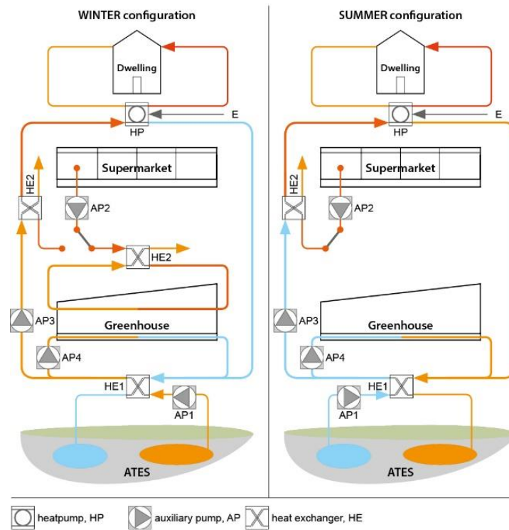
Figure 6. Position of the Auxiliary pumps (AP), Heat exchangers (HE) and Heat Pumps (HP) within the local energy system for both system configurations.
