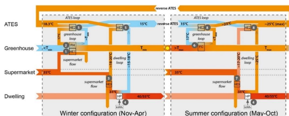
Figure 5. Abstract representation of the thermal energy flows in scenario 2a–d: the local system. Relevant medium/component temperatures are mentioned where ~ indicates an estimated temperature. FH = floor heating, FC = floor cooling, HE = heat exchanger. The ATES reverses at the beginning of May, when the cooling season starts and at the end of October, when the heating season starts. The temperature of the warm well of the ATES is assumed to drop with 3 °C between seasons (see Section 2.5.3.).
