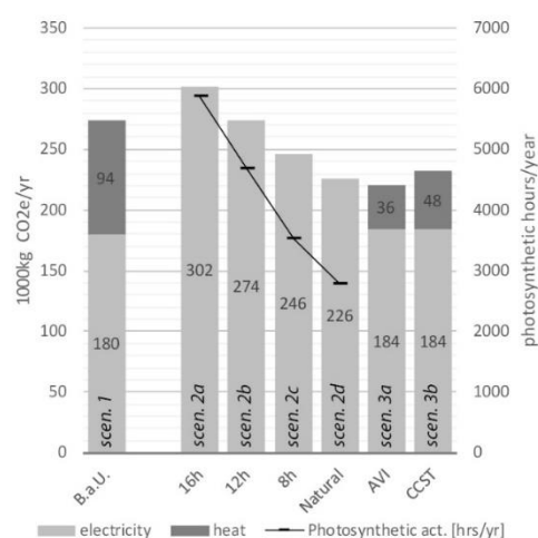
Figure 8. Scenario analysis: BAU, local energy system (scen. 2a–d), district heating method (3a,b). AVI = waste incineration based district heating system, CCST = power plant waste heat based district heating system.
