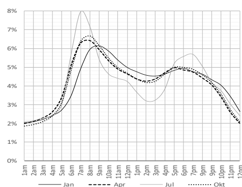
Figure 2. For exemplary purposes: 24 h gas demand curve for an average household in NL, based on Liander data. The % represents the demand for that hour relative to the daily total. Two peaks are evident for each of the four curves: a morning peak when people wake up, turn on the heating and have a shower and an afternoon peak, when people tend to cook dinner (on gas stoves) and switch on the heating (again).
