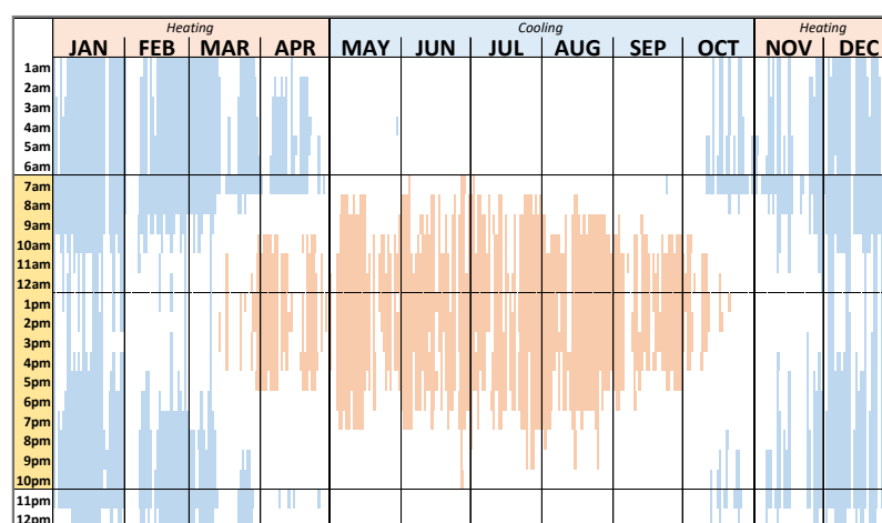
Figure 4. Indoor Greenhouse temperature (°C). Initial set point temperatures: T_{max} = 28 °C, T_{min-D} = 9 °C, T_{min-P} = 12 °C. Blue indicates that T_{min} has been reached or surpassed, red indicates that T_{max} has been reached or surpassed and white indicates that the GH indoor temperature is within desirable range. The yellow hatched hours indicate the photoperiod (PP) timeslot.
