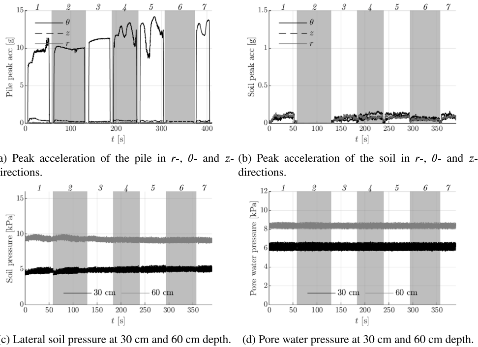
Fig. 17. Pile and soil response data as measured during tests in soil preparation 3.
