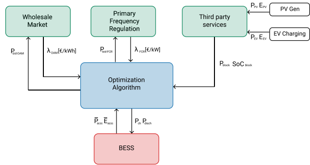
FIGURE 8. The algorithm’s block structure shows the exchange of information among the different modules: Wholesale market, primary frequency regulation, third party operations and the BESS.
