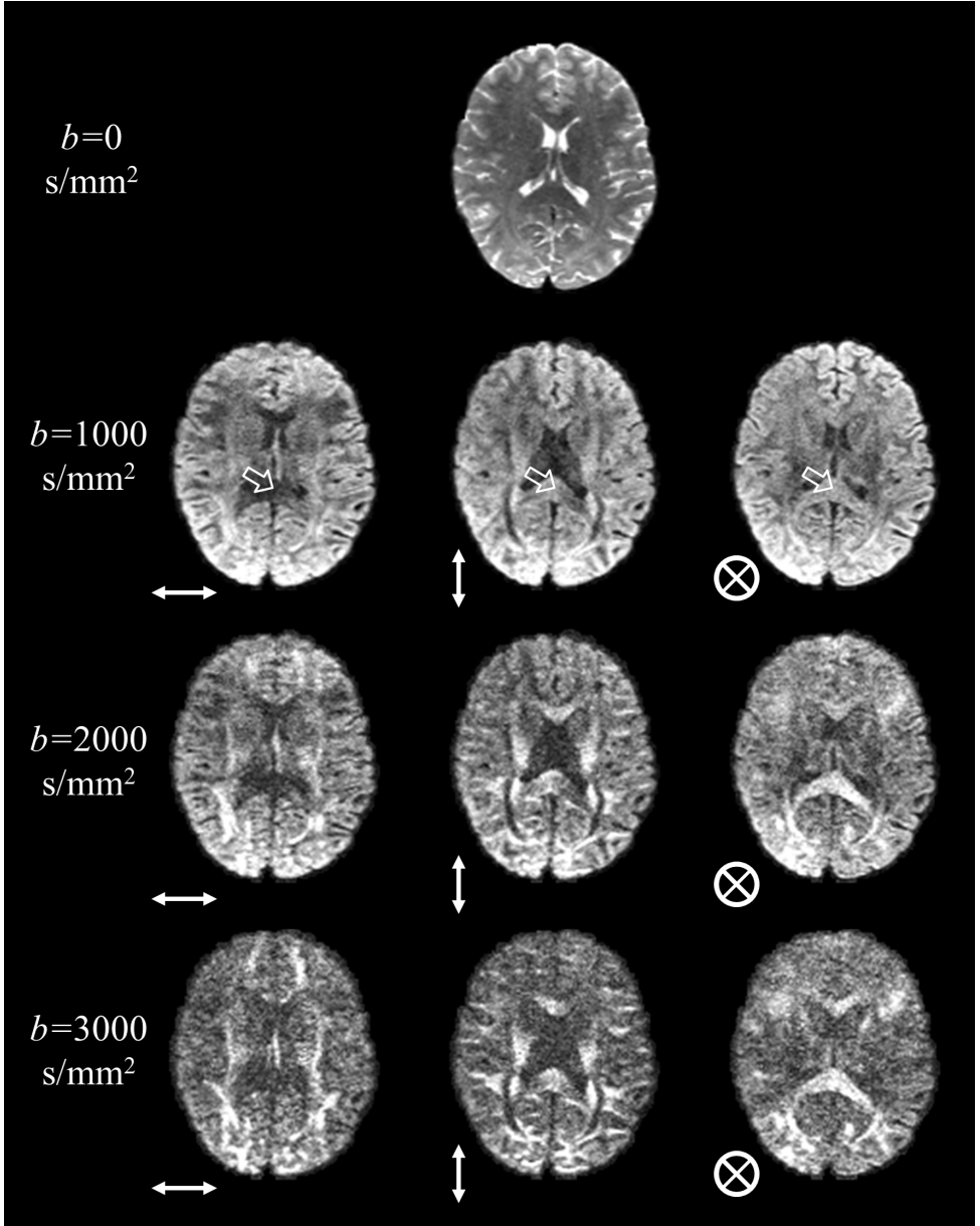
Figure 1.6: Axial slices of diffusion-weighted images with diffusion-sensitizing gradients in different orientations (x, y and z, from left to right) and different diffusion-weighting ( b -value = [0, 1000, 2000, 3000] s/mm 2 ). Images based on DW-MRI data from [13].
