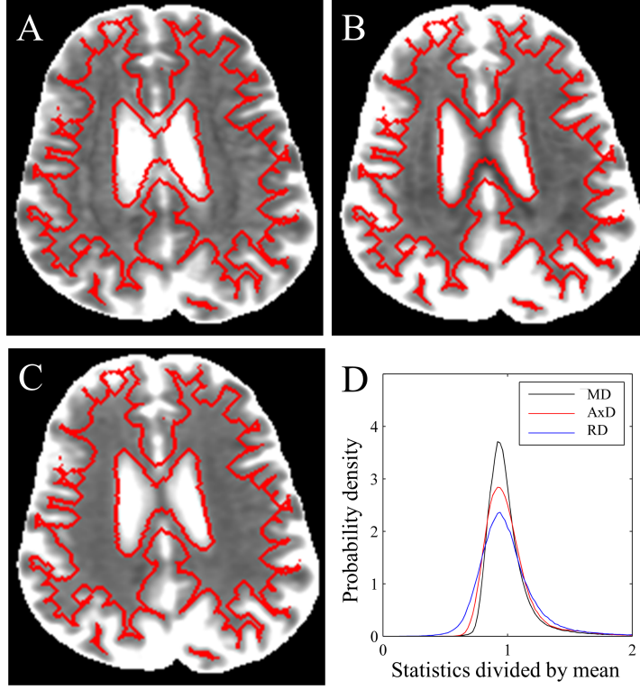
Figure 3.2: Transversal slices from an asymptomatic 65-years old male brain with contours of a white matter segmentation in red. The white matter segmentation was obtained using a kNN tissue segmentation method [25]. A) Axial diffusivity (AxD). B) Radial diffusivity (RD). C) Mean diffusivity (MD) of the diffusion tensor. The images are scaled between zero and two times the mean value of each diffusivity statistic. The mean values of AxD, RD and trace are computed from all voxels in the whole-brain white matter segmentation and are 1.1 \cdot 10^{-3} \text{ mm}^2/\text{s} , 0.69 \cdot 10^{-3} \text{ mm}^2/\text{s} and 0.83 \cdot 10^{-3} \text{ mm}^2/\text{s} respectively. D) Histograms of the AxD, RD and trace after dividing each statistic by its mean value.
