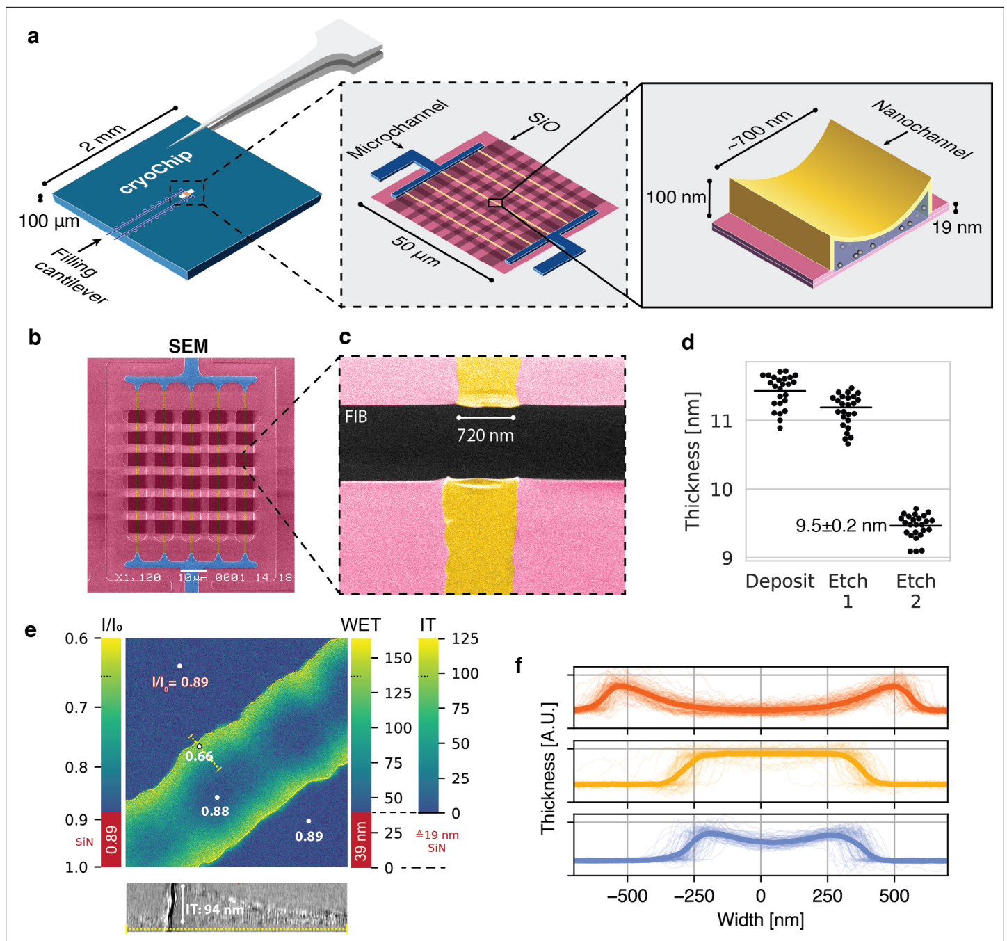
Figure 1. A nanofluidic sample support for cryo-EM. (a) Schematic representation of the MEMS-based cryoChip. The 2 × 2 mm chip base features two microcantilevers for sample filling and air escape. The cantilevers are connected to microchannels leading to a free-standing observation membrane located within an aperture at the chip center (middle inset). A multifurcation connects the microchannels (blue) to an array of five parallel nanochannels (yellow) of approximately 700 nm width and 100 nm height (rightmost inset). The top membrane is smoothly sagging, while the bottom membrane is flat. (b) False-colour scanning electron microscopy (SEM) image of the observation membrane. (c) False-colour SEM image of a single nanochannel with FIB-milled rectangular opening across the observation membrane. (d) Ellipsometric determination of SiN x membrane thickness after deposition and etching steps. (e) Relative thickness map of an ice-filled nanochannel from zero-loss imaging. WET = water-equivalent thickness, IT = ice thickness. The thickness profile correlates with a 2D slice of a tomogram acquired of the same area (bottom). (f) Thickness cross-sections of nanochannels from three chips of the same wafer. Thin lines are individual nanochannel cross-sections measured across a whole chip; thick lines represent their mean.
