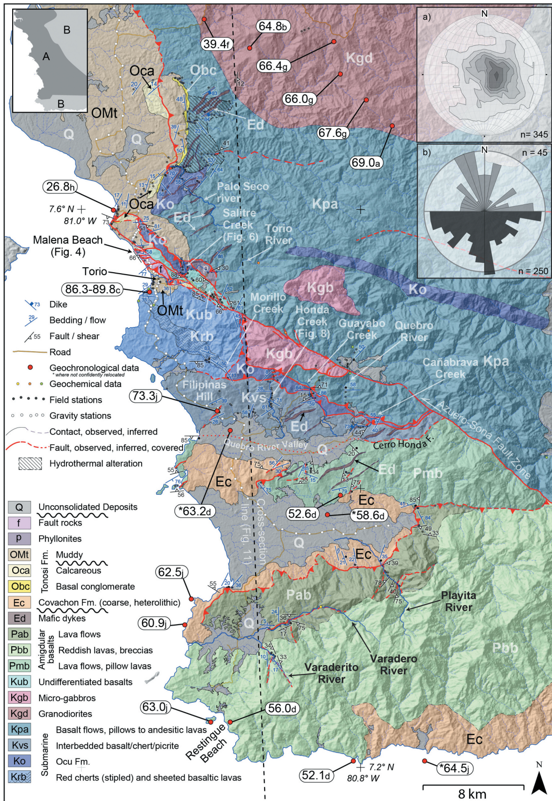
Figure 2. Geologic map of the western half of the Azuero Peninsula. Lower-hemispheric, equal-area projections plots of: A) kamb contours of poles to bedding (2 sigma contour interval), and B) dip direction of joints and dikes (top half-rose, 11% outer perimeter), and faults, foliation and cleavage (bottom half-rose, 8% outer perimeter), see SM2 for raw data. Geochronological ages in millions of years, subscripts indicate author (a: Guidice and Recchi 1969; b: Kesler et al. 1977; c: Kolarsky et al. 1995; d: Hoernle et al. 2002; e: Lissina 2005; f: Tournon and Bellon 2009; g: Montes et al. 2012; h: Kedenburg 2016; i: Ramirez et al. 2016 j: Gazel et al. 2018).
