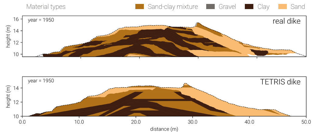
A comparison of the construction history and resulting heterogeneity of an actual river dike (top) and a dike simulated by the TETRIS algorithm. Image by Teun van Woerkom.
