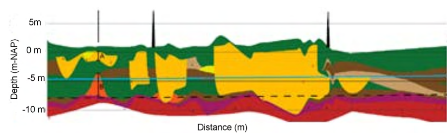
Subsoil profiles from borehole data
