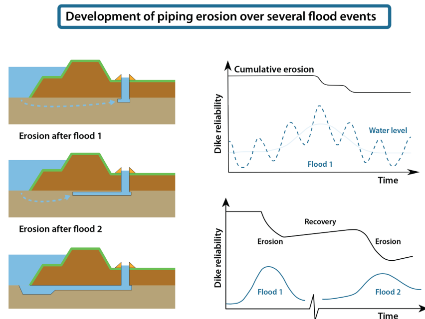
Figure 3: Left: Piping schemes adapted from van Beek (2015) and dike reliability graphs sketched by Joost Pol.
