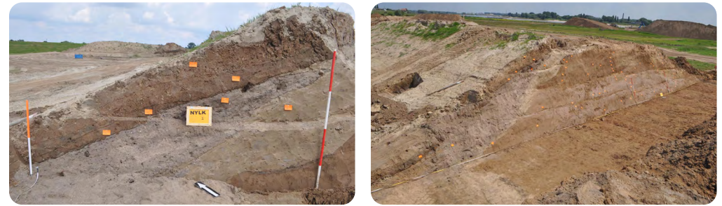
Images of a historical dike, which clearly consists of many different layers of various material types. Photos from Rondags (2019) .
