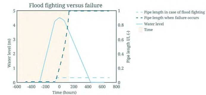
Flood fighting
