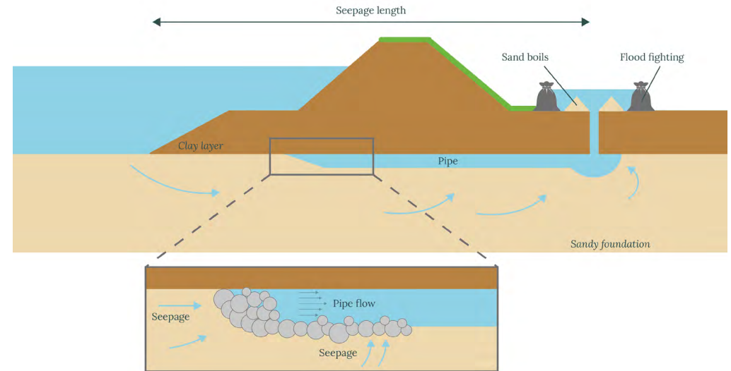
Illustration of the piping erosion processes. Adapted from Robbins & Sharp (2016, Figure 1) .
