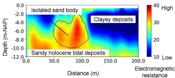
Geophysical measurements
