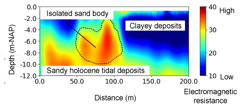
Figure 1: Paleochannel detection with electrical resistivity tomography.
