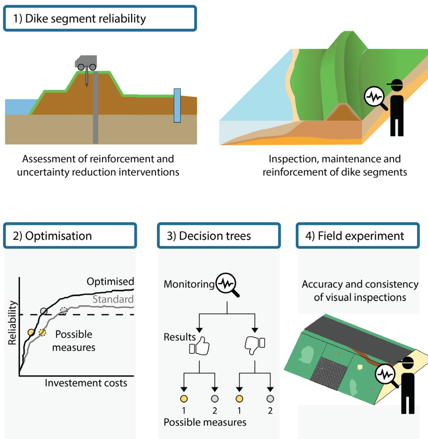
Figure 3: Components of the research relating decisions at a dike section to a whole segment. Figure 3.1 is based on schemes by Wouter Jan Klerk, dike segment scheme prepared by Richard Marijnissen.
