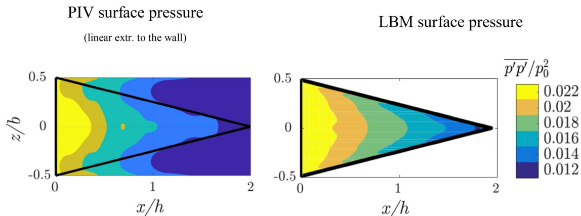
Fig. 13 Intensity of the mean pressure fluctuations \overline{p'p'}/p_0^2 as reported by the authors (Avalone et al. 2018) (corresponding to \overline{p_{rms}^2}/q_\infty^2 in this manuscript). Comparison between the results from the numerical study in the literature and the ones from tomographic PIV in this manuscript
