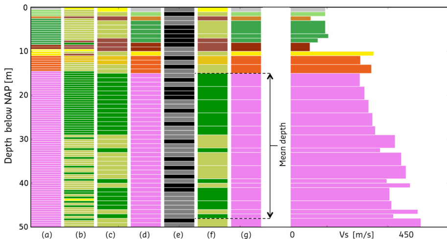
Fig. 14 Example of GeoTOP voxel-stack processing. From left to right: (a) original GeoTOP stratigraphic units; (b) original GeoTOP lithological classes; (c) resampled lithological classes into layers of 1.0 m thickness; (d) resampled stratigraphic units into layers of 1.0 m thickness; (e) random selector used to select the upper (grey) or lower (black) voxel; (f) merged lithological classes with a maximum thickness of 3.0 m; (g) merged stratigraphic units with a maximum thickness of 3.0 m. For the clays (green) of the Peelo Formation (purple), the mean depth of the unit is indicated. Far right: bar graph of the sampled shear-wave velocity profile assigned to the voxels by applying the routine from Fig. 15 to voxel-stacks (f) and (g)
