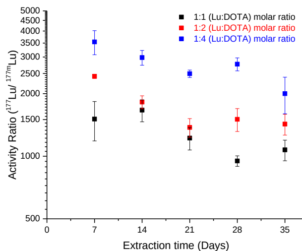
Figure 4: The ^{177}\text{Lu}/^{177\text{m}}\text{Lu} activity ratio obtained during the successive LLE of free ^{177}\text{Lu} ions from the [^{177\text{m}}\text{Lu}]\text{Lu} -DOTA complex. The experiments were performed with three Lu: DOTA molar ratios, (1:1) in black, (1:2) in red and (1:4) in blue. The data points represent the average \pm STD of three experiments, the individual error in measurements due to counting statistics is less than 5%.
