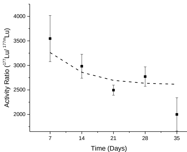
Figure 7: The ^{177}\text{Lu}/^{177\text{m}}\text{Lu} activity ratio obtained at different elution time when the LLE is performed with [ ^{177\text{m}}\text{Lu} ]Lu-DOTA complex synthesized in a molar ratio 1:4. The data points represent the experimentally observed ratios, while the dotted line represents the expected activity ratios with 60% ^{177}\text{Lu} extraction efficiency and 0.002% ^{177\text{m}}\text{Lu} ions leakage.
