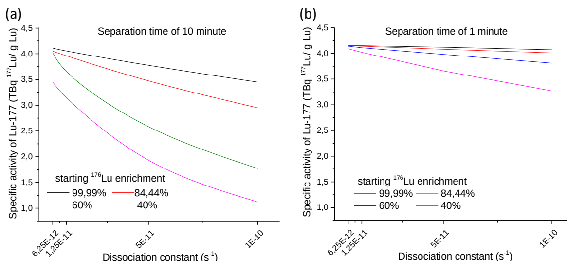
Figure 6: The specific activity of the produced ^{177}\text{Lu} as a function of dissociation rate constant for different ^{176}\text{Lu} enrichment containing targets and (a) a ^{177\text{m}}\text{Lu} - ^{177}\text{Lu} separation time of 10 minutes, (b) ^{177\text{m}}\text{Lu} - ^{177}\text{Lu} separation time of 1 minute.
