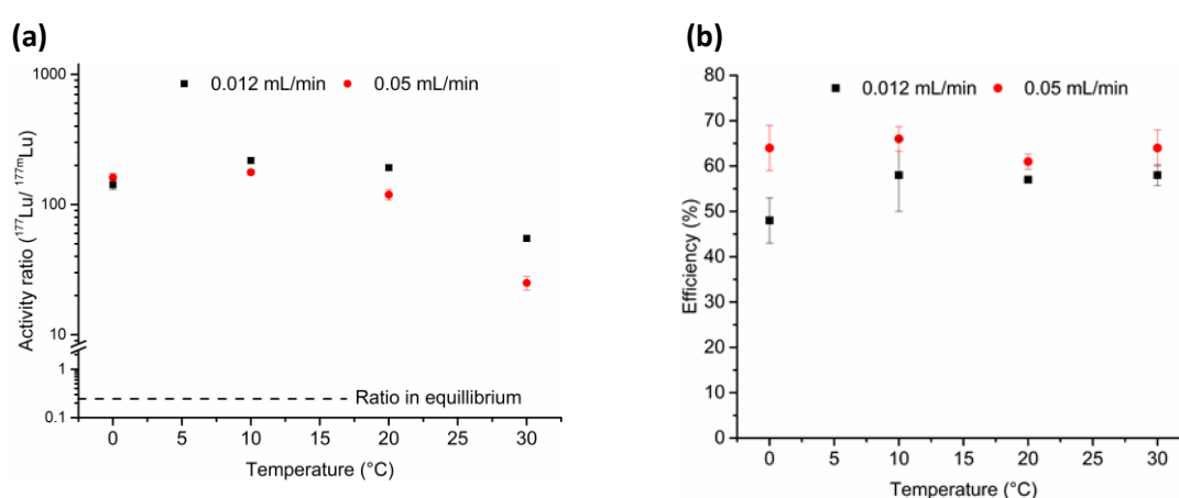
Figure 3: Effect of temperature and flow rate on efficiency (a) Effect of temperature on the ^{177}\text{Lu}/^{177\text{m}}\text{Lu} activity ratio at different flow rates (■ 0.012\text{ mL/min} and ● 0.05\text{ mL/min} ). (b) Effect of temperature on the efficiency of separation at different flow rate (■ 0.012\text{ mL/min} and ● 0.05\text{ mL/min} ).
