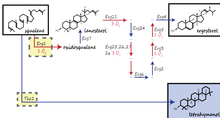
Figure 3.1: Schematic overview of ergosterol and tetrahymanol synthesis pathways. Erg1, Erg7, Erg24, Erg25, Erg26, Erg27, Erg6, Erg2, Erg3, Erg5, and Erg4, native S. cerevisiae enzymes involved in the oxygen-dependent synthesis of ergosterol from squalene. Thc1, squalene tetrahymanol cyclase from Tetrahymena thermophila . Oxidosqualene, epoxidation product of squalene, formed by Erg1. Lanosterol, first tetracyclic compound in fungal ergosterol synthesis. For oxygen-dependent reactions, the number of moles of oxygen required is indicated. Dashed boxes represent enzymes whose expression levels were modified in this study.
