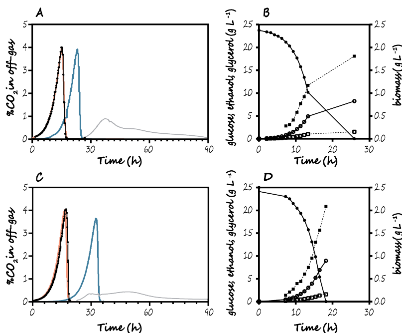
Figure 3.3: Anaerobic sequential batch bioreactor (SBR) cultivation of S. cerevisiae strains IMX585 and IMX1438 with sterol supplementation. All panels represent data from a single representative SBR experiment performed at 30 °C on SMD-urea without pH control. Data from replicate experiments are shown in Figure S4. (A and B) Reference strain IMX585. (C and D) Strain IMX1438 ( sga1Δ::TtTHCI ). (A and C) Percentages of CO 2 in off-gas during the initial batch cycle without anaerobic growth factors (grey line) and during the first (blue line), second (black line and dots), and third (red line) subsequent SBR cycles on SMD-urea supplemented with Tween 80 and ergosterol. (B and D) Concentrations of glucose (closed circles), biomass (closed squares), ethanol (open circles), and glycerol (open squares) in the second SBR cycle.
