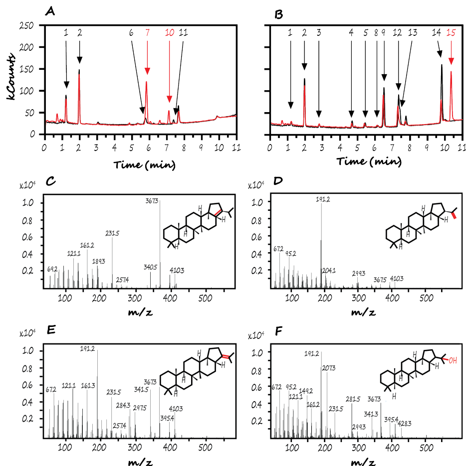
Figure 4.3: Gas chromatography-mass spectrometry (GC-MS) analysis of triterpenoid fractions of anaerobically grown yeast biomass. Anaerobic cultures were harvested in early stationary phase. Triterpenoids were extracted for GC-MS analysis and injected immediately (black lines) or after silylation (red lines). (A) S. cerevisiae CEN.PK113-7D grown anaerobically on medium supplemented with Tween 80 and ergosterol, (B) Sch. japonicus CBS5679 was grown on medium supplemented with only Tween 80. Numbers indicate the following compounds: 1, squalene; 2, 5 \alpha -cholestane (internal standard); 3, squalene epoxide; 4, hop-17(22)-ene; 5, unidentified component; 6, ergosterol; 7, ergosterol-TMS-ether; 8, unidentified component; 9, unidentified component, possibly a tricyclic intermediate; 10, lanosterol-TMS-ether; 11, lanosterol; 12, hop-22(29)-ene (diploptene); 13, hop-21(22)-ene; 14, hopan-22-ol (diplopterol); 15, hopan-22-ol-TMS-ether. (C-F) Mass spectra and structures of identified hopanoid compounds in the triterpenoid fraction of anaerobically grown biomass of Sch. japonicus . (C) Hop-17(21)-ene, (4). (D) Hop-22(29)-ene, (12). (E) Hop-21(22)-ene, (13). (F) Hop-22-anol (diplopterol), (14).
