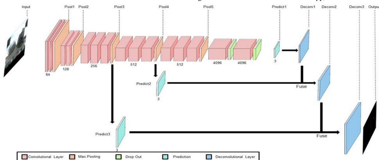
Figure 7. FCN Architecture
