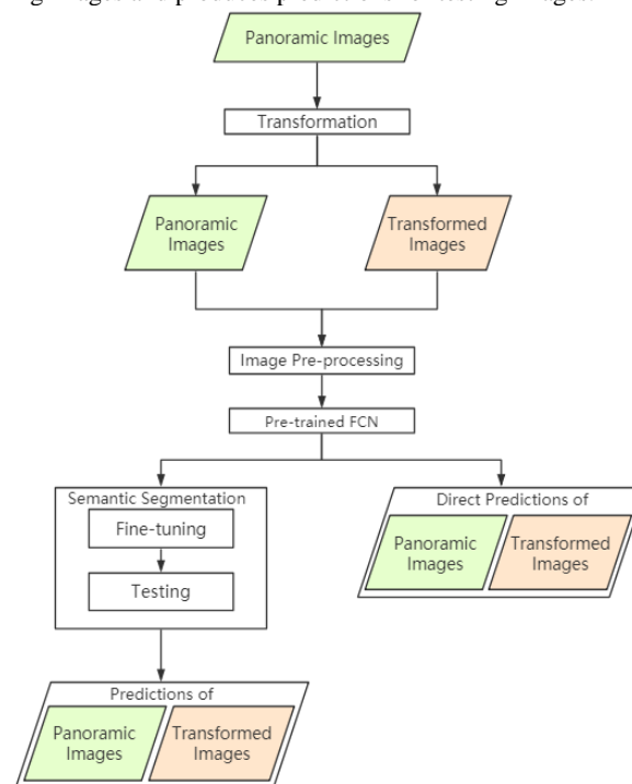
Figure 1. Workflow of the proposed street furniture identification.
