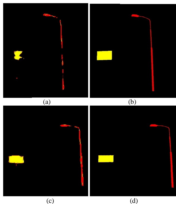
Figure 11. Predictions of fine-tuning. (a) (b) The prediction and labeled ground truth of panoramic images. (c) (d) The prediction and labeled ground truth of transformed images.
