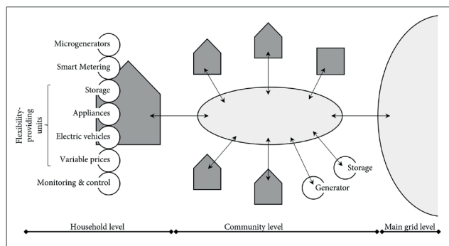
Figure 1-1: Schematic overview of a smart grid system
