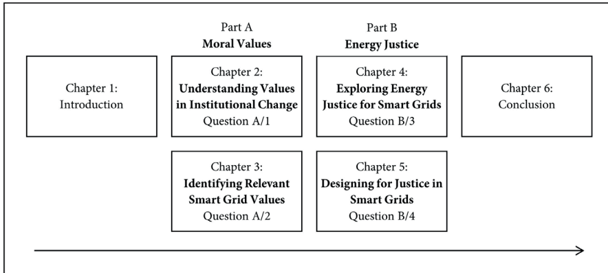
Figure 1-2: Dissertation outline
