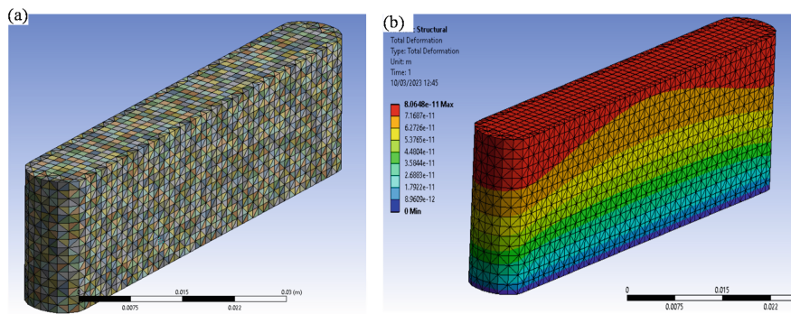
Fig. 5. The results of mesh model generation. a Mesh full pier model solved successfully within ANSYS Workbench, and b Triumphal internal computation within ANSYS Workbench
