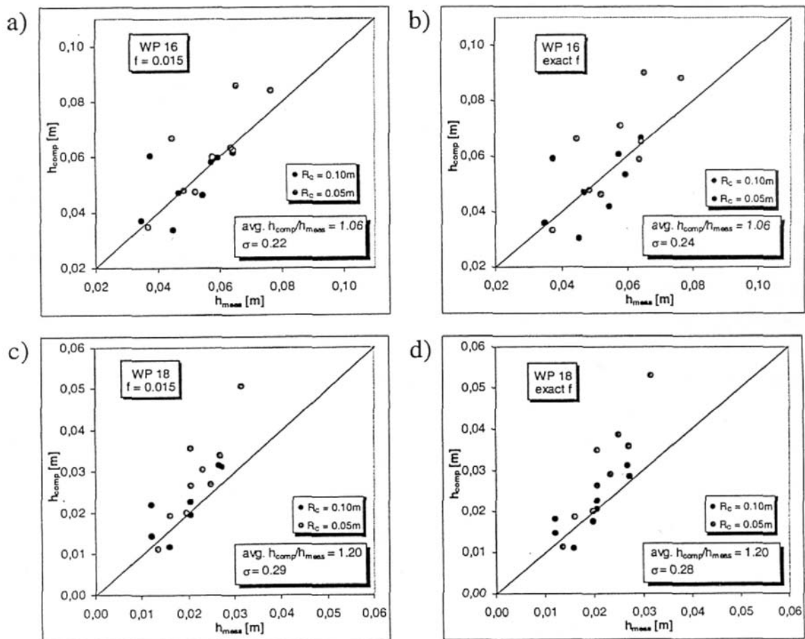
Figure 60: Comparison of computed and measured layer thicknesses.
