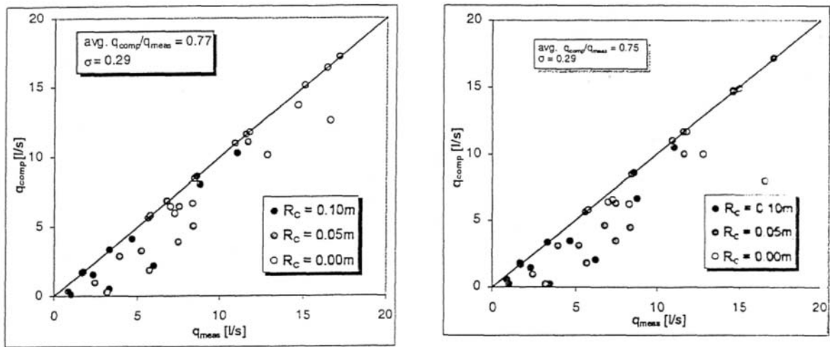
Figure 59: Ratio of measured to computed overtopping rates for (left) computed regular waves by ODIFLOCS and (right) measured regular waves at the toe of the dike in the physical model.
