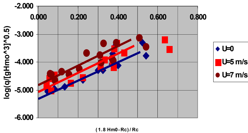
Figure 50: \log(Q/(gH_{m0})^{1.5}) as function of (RuH-Rc)/Rc and wind speed.
