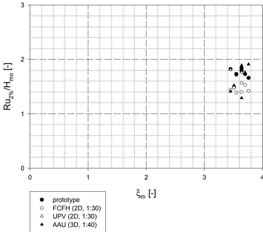
Figure 45: Comparison of prototype measurement and laboratory test results
