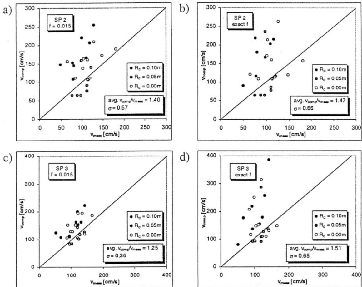
Figure 61: Comparison of computed and measured overtopping velocities.
