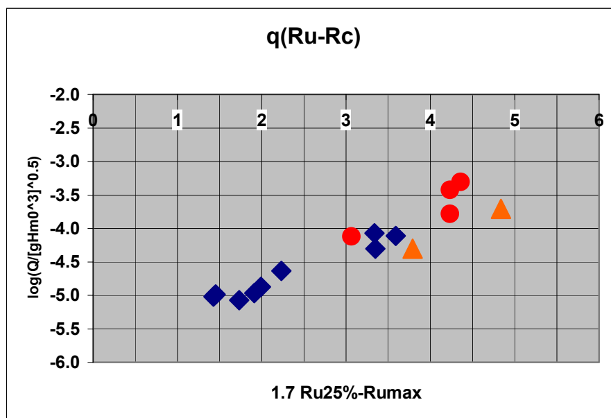
Figure 26: \log(Q/H_{mo}^{1.5}) as function of (Ru-Rc)
