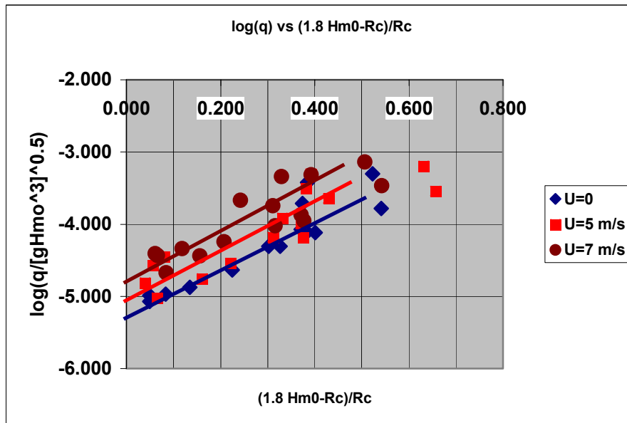
Figure 27: \log(Q/H_{m0}^{1.5}) as function of \{(RuH-Rc)/Rc\} and windspeed.
