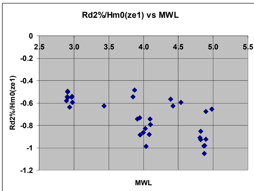
Figure 25: Rd_{2\%}/H_{m0} as function of MWL .
