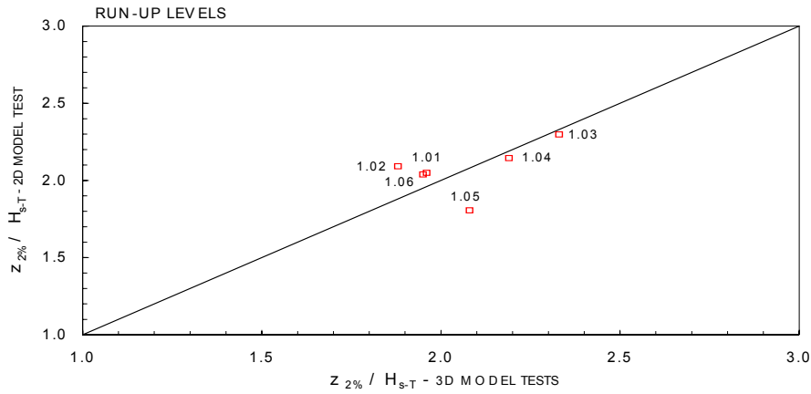
Figure 43: Comparison between wave run-up levels measured in 6 storms in 2D model tests and in 3D model tests.
