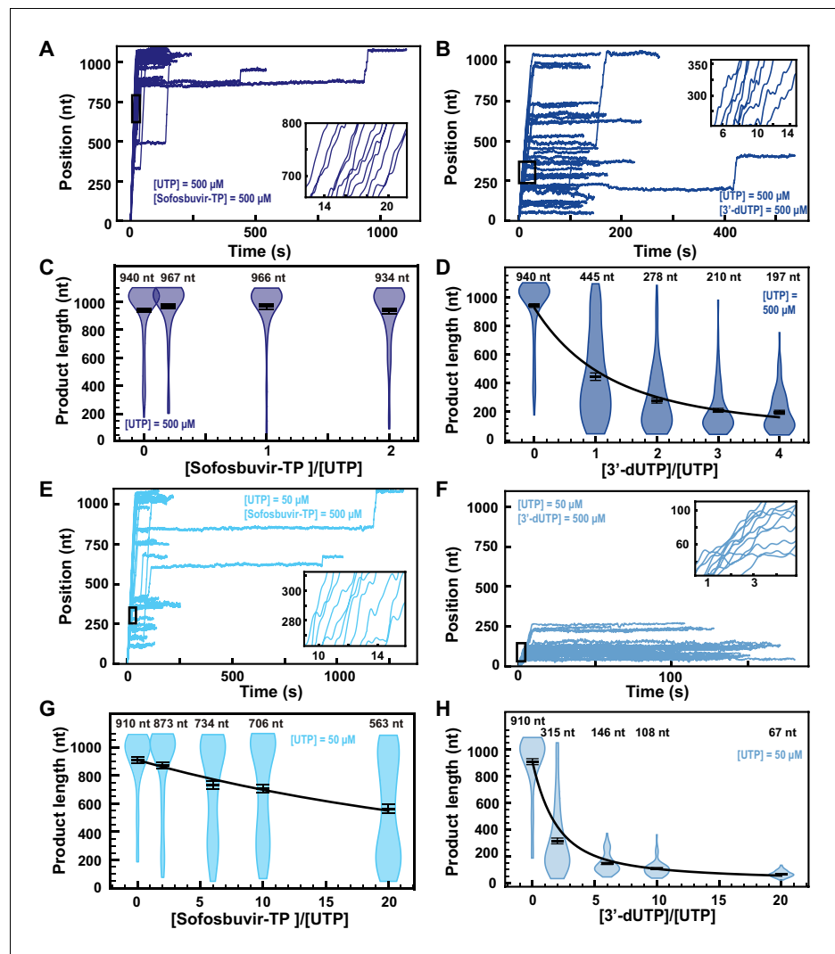
Figure 5. Sofosbuvir-TP is a poor SARS-CoV-2 polymerase inhibitor in contrast with 3'-dUTP. (A, B) SARS-CoV-2 polymerase activity traces for 500 \mu\text{M} NTPs and 500 \mu\text{M} of either (A) Sofosbuvir-TP or (B) 3'-dUTP. (C, D) SARS-CoV-2 polymerase product length using the indicated concentration of UTP, 500 \mu\text{M} of other NTPs, as a function of either (C) [Sofosbuvir-TP]/[UTP] or (D) [3'-dUTP]/[UTP]. The mean values are indicated above the violin plots, and represented by horizontal black thick lines flanked by one standard deviation error bars extracted from 1000 bootstraps. (E, F) SARS-CoV-2 polymerase activity traces in the presence of 50 \mu\text{M} of UTP, 500 \mu\text{M} of all other NTPs, and 500 \mu\text{M} of either (E) Sofosbuvir-TP or (F) 3'-dUTP. (G, H) SARS-CoV-2 polymerase product length using 50 \mu\text{M} UTP, 500 \mu\text{M} of other NTPs, as a function of either (G) [Sofosbuvir-TP]/[UTP] or (H) [3'-dUTP]/[UTP]. The mean values are indicated above the violin plots, and represented by horizontal black thick lines flanked by one standard deviation error bars extracted from 1000 bootstraps. In (D, G, H), the solid line is the fit of the terminator effective incorporation rate (see Materials and methods). In (A, B, E, F), the insets are a zoom-in of the replication traces captured in the black square.
