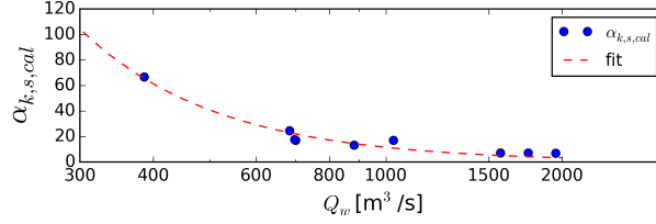
Figure 3: Power function obtained between the calibrated value of \alpha_{k,s} obtained for each scenario and the associated flow-rate Q_w .
