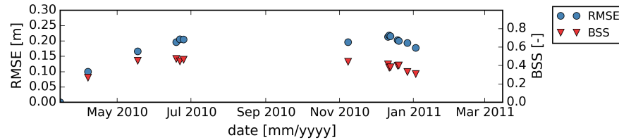
Figure 7: Time-series of RMSE and BSS computed on bed topography, taking account of sediment sorting (scenario A), from March 15 th 2010 to January 3 rd 2011.
