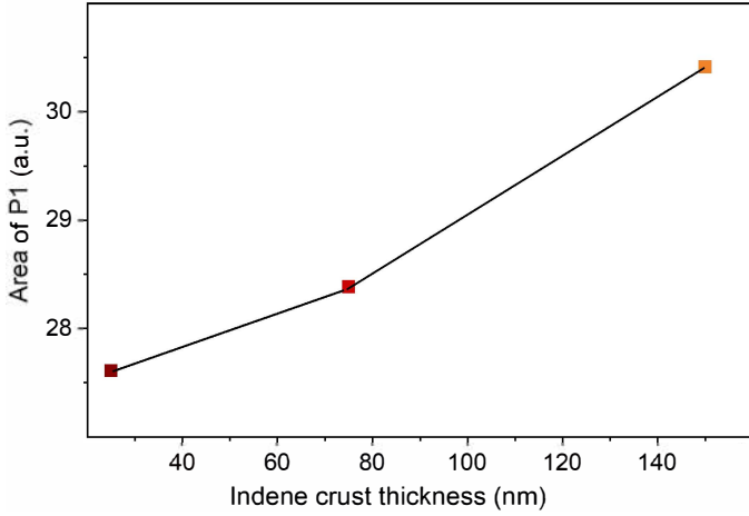
Fig. 9. Area of the P_1 desorption peak of methane versus indene layer thickness.
