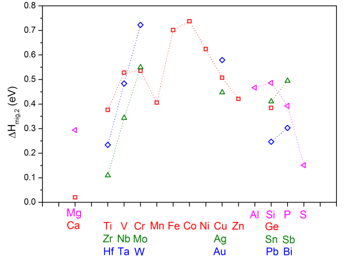
FIG. 6. Migration enthalpy \Delta H_{\text{mig},2} of impurity elements calculated with Eq. (15), arranged by row and column of the periodic table: row 3 of the periodic system (purple triangles), row 4 of the periodic system (red squares), row 5 of the periodic system (green triangles), and row 6 of the periodic system (blue diamonds). Dashed lines, between neighboring impurities, are guides to the eyes only.
