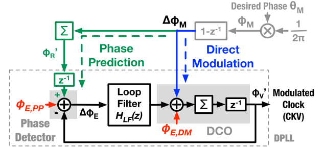
Fig. 2. Discrete-time domain model of an ideal PLL-based phase modulator with a two-point modulation. The gains of DCO and phase detector, respectively, K_{DCO} and K_{PD} , are implied as normalized, as in [27], hence hidden.
