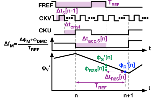
Fig. 8. Predicting \phi'_S by subtracting \phi_{R2S} from \phi'_R , in face of the non-uniform CKU.
