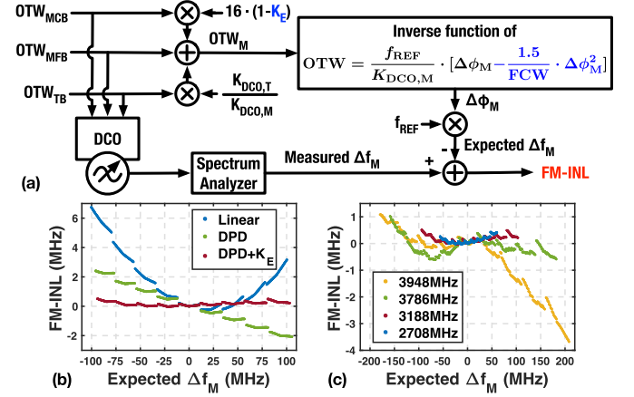
Fig. 18. DCO FM-INL: (a) Measurement setup, (b) measured results with different DCO linearization settings when f_0 = 3188 MHz, and (c) measured results with the proposed phase-domain DPD and the same K_E = 0.023 at multiple f_0 's.
