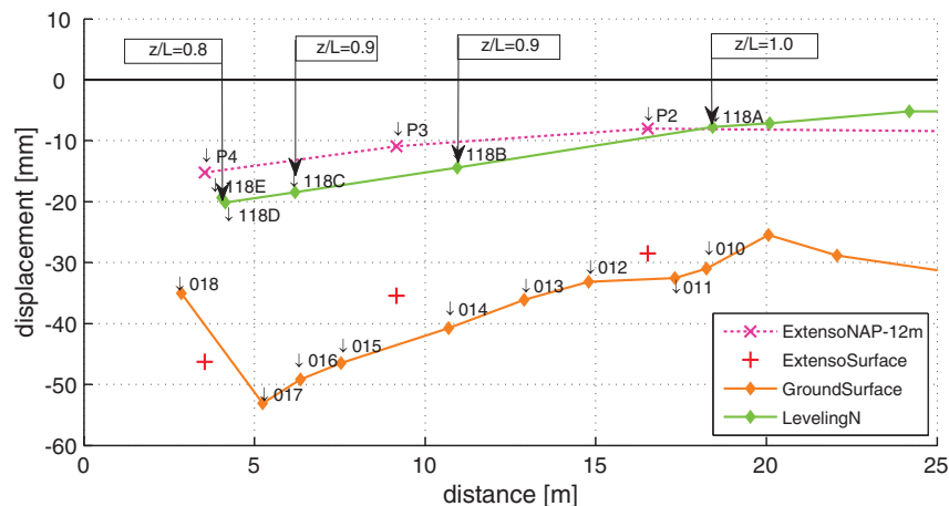
Fig. 20. (Color) Ground and building displacements for Ferdinand Bolstraat 118 (Ceintuurbaan) with distance from the deep excavation, showing interaction levels ( z/L ) derived from measurements
