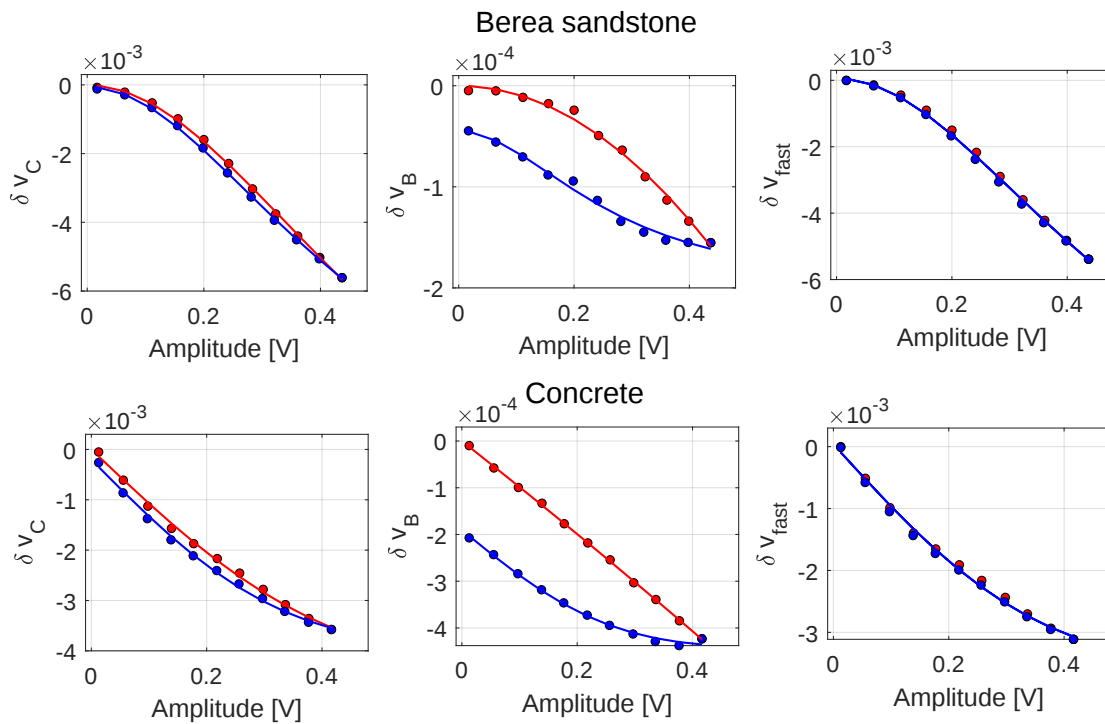
Figure 3. Velocity variations vs. conditioning strain. \delta v_C and \delta v_B are the conditioned and baseline velocity variations, respectively. \delta v_{\text{fast}} is the fast dynamic contribution to the velocity variation (see Equation (5)). Red symbols refer to loading (drive amplitude increases), while blue ones to unloading (drive amplitude decreases). Data reported refer to measurements performed at T = 283 K. Here, the x-axes (strain) correspond to the output amplitude (in volts) defined by Equation (3), when A_{\text{drive}} = A_{\text{cnd}} .
