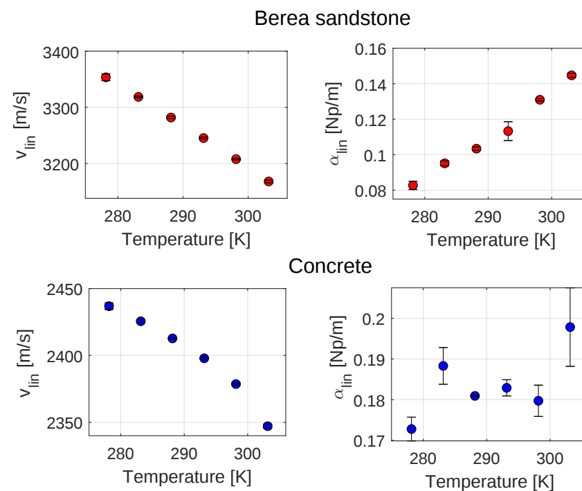
Figure 4. Linear viscoelastic parameters vs. temperature: velocity ( left ) and damping ( right ). Data are averaged over repetitions of the experiment and the errorbar is given by the semidisperson.
