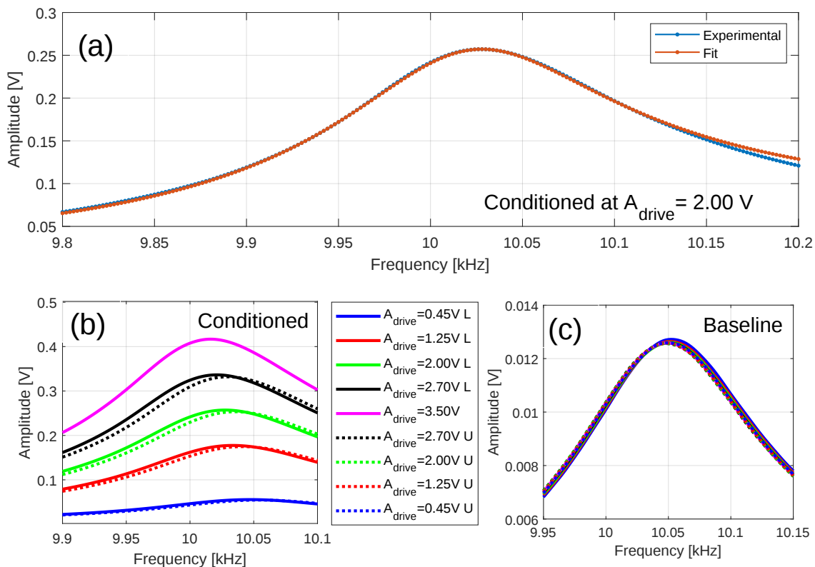
Figure 2. Spectra for concrete at T = 298 \text{ K} . (a) Superposition of experimental data and fit (using Equation (2)) for a given drive amplitude. (b) Conditioning spectra for selected drive amplitudes. (c) Baseline spectra for the same drive amplitudes as in (b). Colors indicate the drive amplitudes, solid lines refer to loading, and dashed lines refer to unloading. For the description of subplots (b,c), refer to Section 3.
