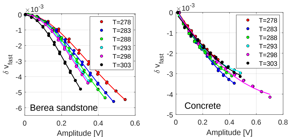
Figure 5. Nonlinear fast velocity variations vs. strain at different temperatures. Here, the x-axes (strain) correspond to the output amplitude (in volts) defined by Equation (3), when A_{\text{drive}} = A_{\text{cnd}} .
