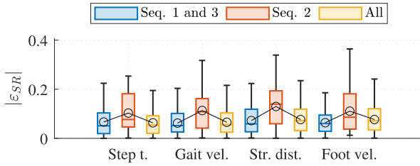
Fig. 12. Distribution of |\epsilon_{SR}| for the different gait parameters considering the multipath effect: small for Gait Sequences 1 and 3 and strong for Gait Sequence 2. The mean of |\epsilon_{SR}| is represented with black circles.
